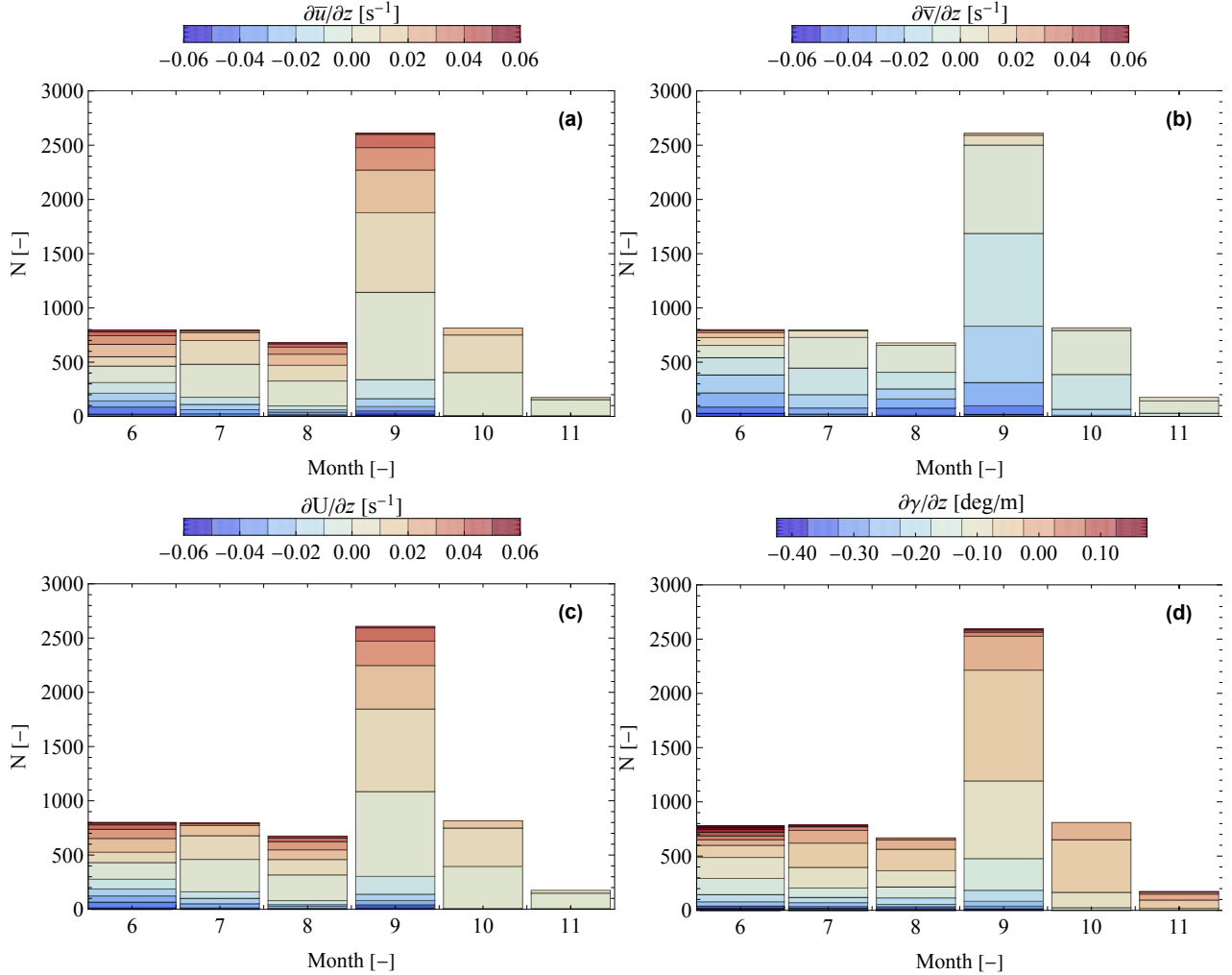
Figure 4. Bar chart of the distribution of the estimated gradients (a) \frac{\partial \bar{u}}{\partial z} and (b) veer \frac{\partial \bar{v}}{\partial z} along with the corresponding shear (c) and veer (d) of the wind profile along the top part of the wind turbine rotor for different 10-minute periods over different months.
