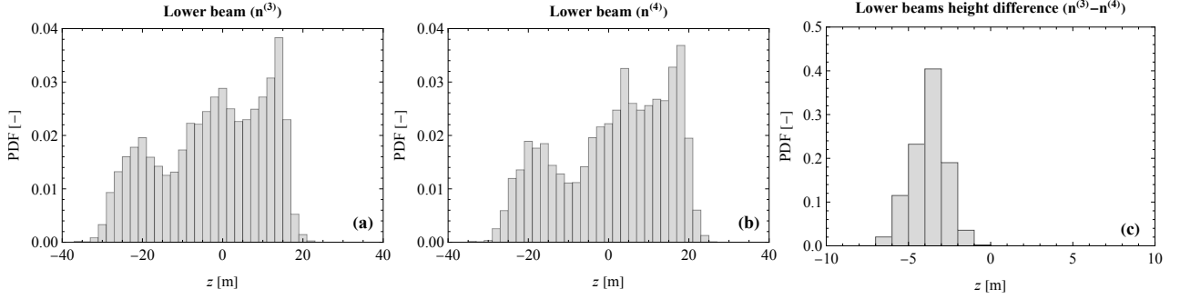
Figure B1. Probability density function of the height z of the range gate measurement of 2.6 D of the left (a) and right (b) lower beams of the nacelle-mounted Doppler lidar in relation to the hub-height and (c) of the difference between the two.
