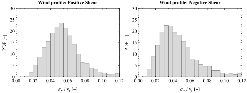
Figure D1. Probability density function of the average standard deviation of the radial speeds measured by the nacelle-mounted wind lidar at the furthest range gates and at the two lower lines of sight for the cases of wind profiles with positive (left) and negative (right) shear.
