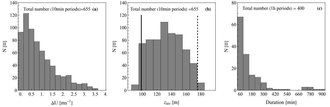
Figure 6. Histograms of (a) the wind speed difference ( \Delta U ) between the maximum and the minimum wind speed along the wind vertical profile, (b) the height of the wind speed inversion ( z_{inv} ) and (c) the duration of periods in which either wind speed inversion or negative shear were identified. The solid and dashed vertical lines in (b) denote the hub height and top height of the rotor.
