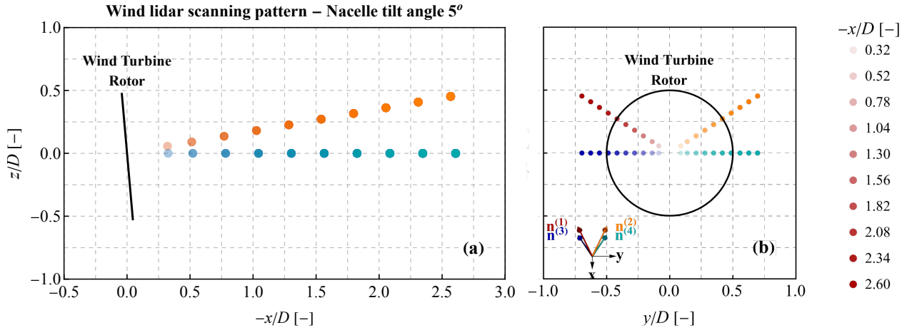
Figure 2. Scanning pattern of the nacelle-mounted wind lidar when the tilt of the floating offshore wind turbine is equal to 5^\circ , corresponding to the wind speed ranges 8.5 - 9.5 \text{ ms}^{-1} and 12.5 - 13.5 \text{ ms}^{-1} . The two lower beams (denoted as n^{(3)} and n^{(4)} ) are almost horizontal when the pitch angle is approximately equal to 5^\circ . The x -axis is parallel to the yaw direction and pointing downwind.
