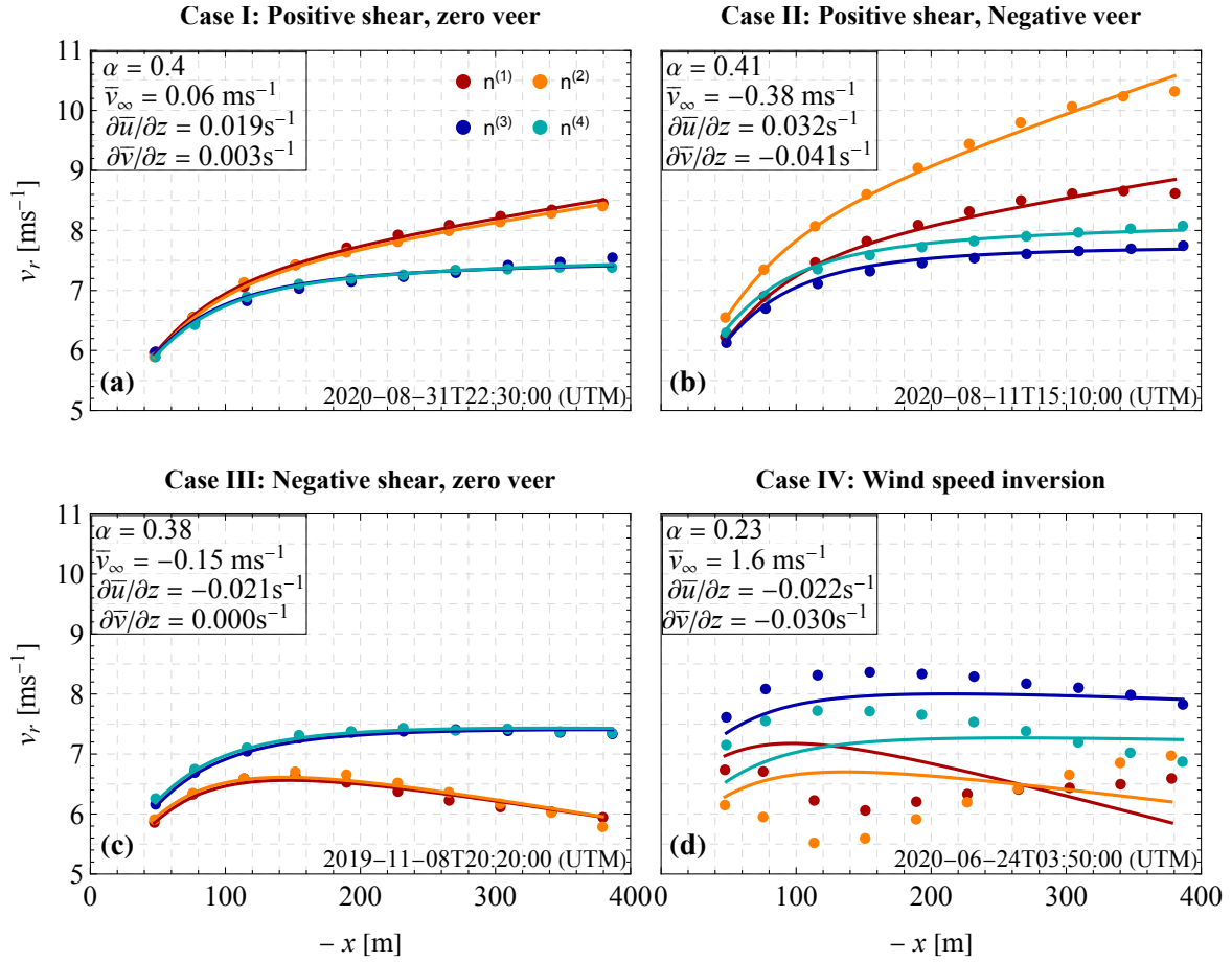
Figure 3. Example of the mean radial speed measurements (presented in dots) of a nacelle-mounted wind lidar acquired over four different line of sights (i.e. n^{(i)} , with i=1,2,3 and 4) and upwind distances (i.e. 50 – 400 m) during 10-minute periods when the wind profile was characterized by positive \frac{\partial \bar{u}}{\partial z} and zero \frac{\partial \bar{v}}{\partial z} (a), positive \frac{\partial \bar{u}}{\partial z} and negative \frac{\partial \bar{v}}{\partial z} (b), negative \frac{\partial \bar{u}}{\partial z} and zero \frac{\partial \bar{v}}{\partial z} (c) and by wind speed inversion (d). The information of the upwind conditions ( \bar{v}_\infty , \frac{\partial \bar{u}}{\partial z} and \frac{\partial \bar{v}}{\partial z} ) and the induction factor a of the wind turbine of each example is presented the corresponding plot. The solid lines correspond to the estimated distribution of the line-of-sight velocities using Eq. 1.
