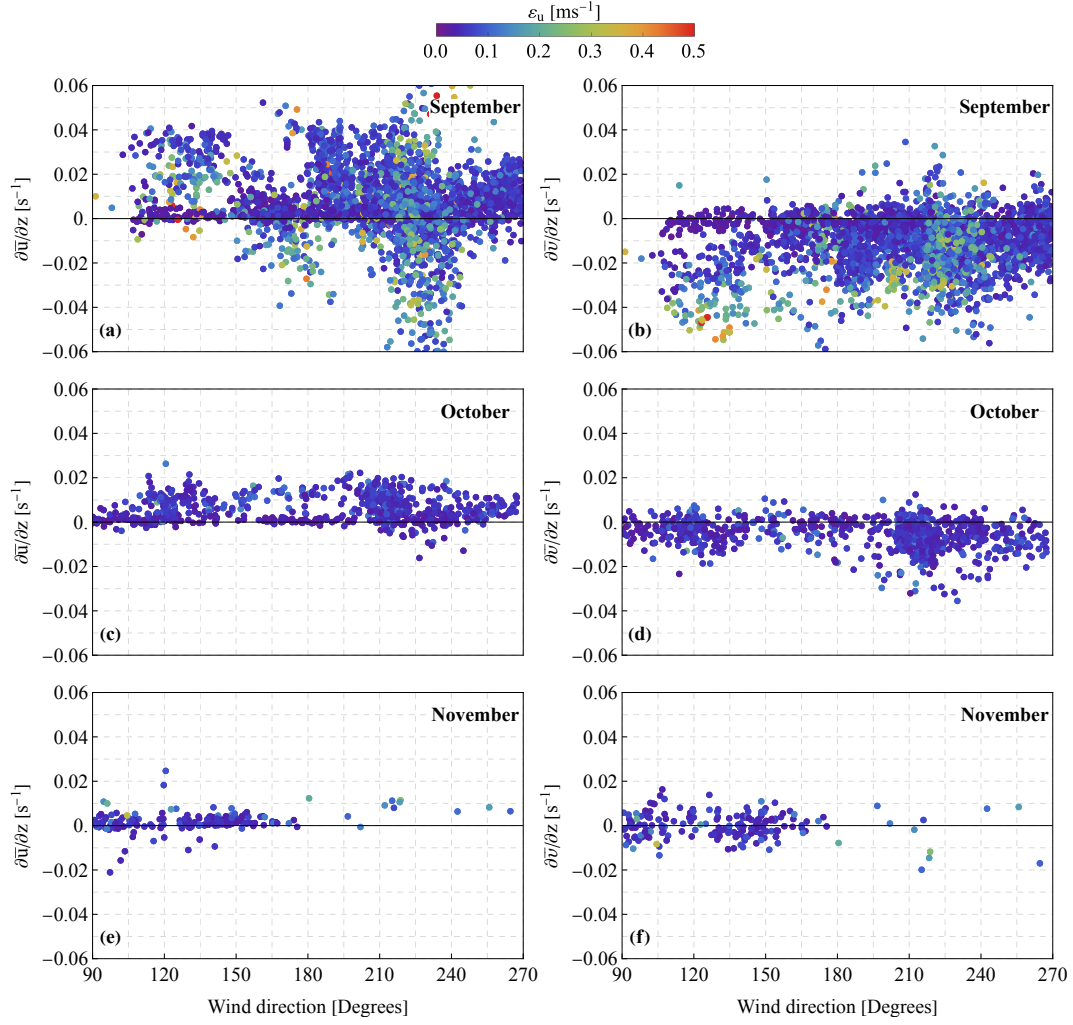
Figure A2. Wind gradients \frac{\partial \bar{u}}{\partial z} and \frac{\partial \bar{v}}{\partial z} values for different 10-minute periods versus wind direction for the months September ((a) – (b)), October ((c) – (d)) and November ((e) – (f)).
