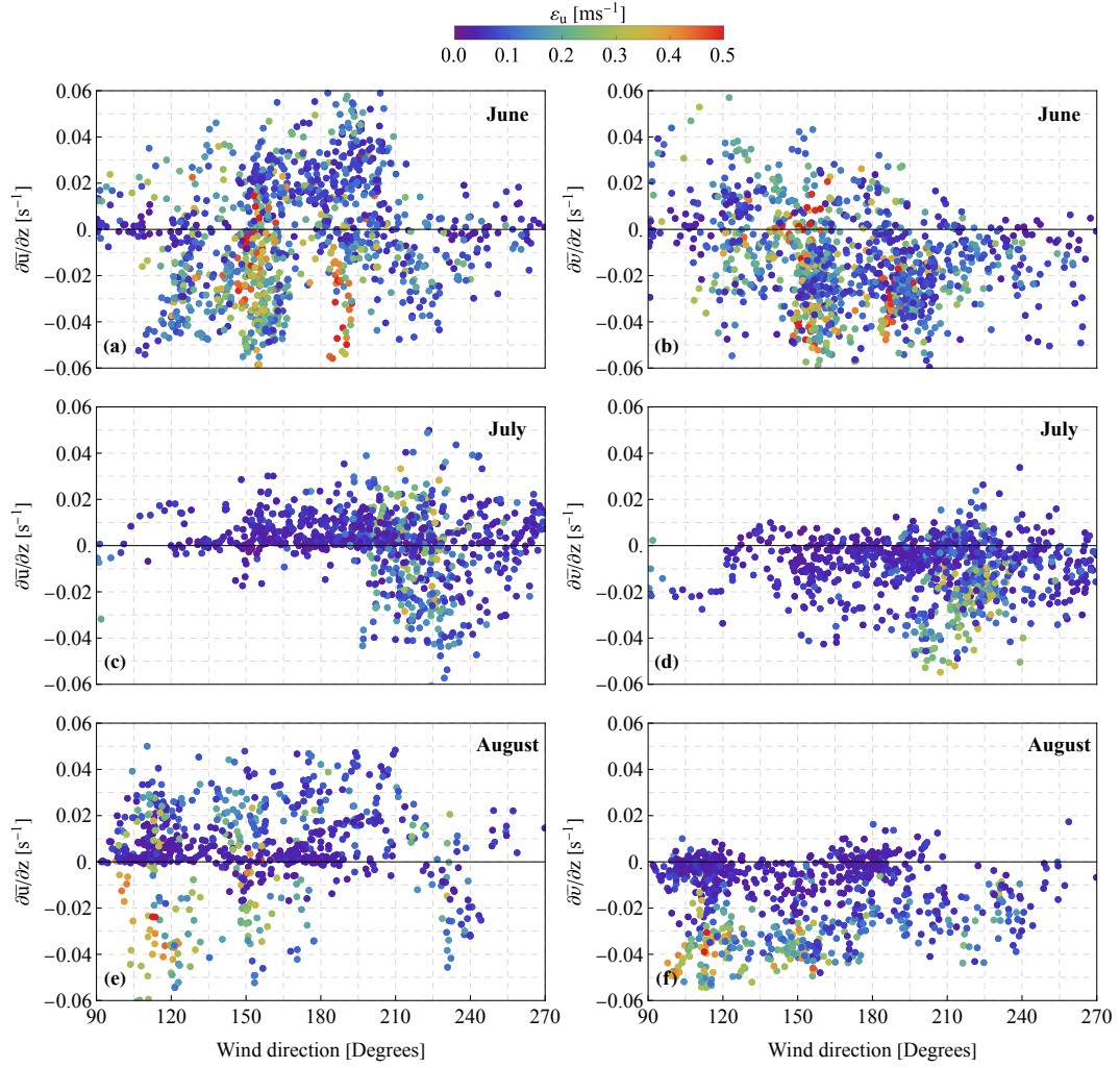
Figure A1. Wind gradients \frac{\partial \bar{u}}{\partial z} and \frac{\partial \bar{v}}{\partial z} values for different 10-minute periods versus wind direction for the months June ((a) – (b)), July ((c) – (d)) and August ((e) – (f)).
