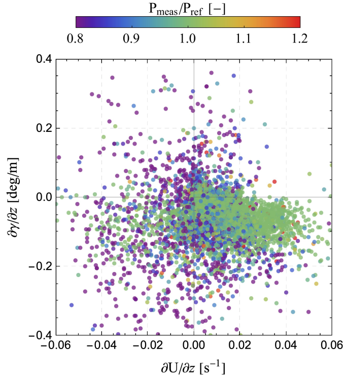
Figure C1. Power ratio, measured power divided by the theoretical produced power using a hub height wind speed, for different wind shear ( \frac{\partial U}{\partial z} ) and veer ( \frac{\partial \gamma}{\partial z} ) values estimated over 10-minute periods.
