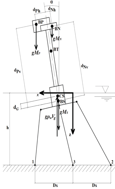
Figure 2. Offshore wind turbine floating platform. Figure reproduced from Betti et al. (2014), where all symbols are defined.
