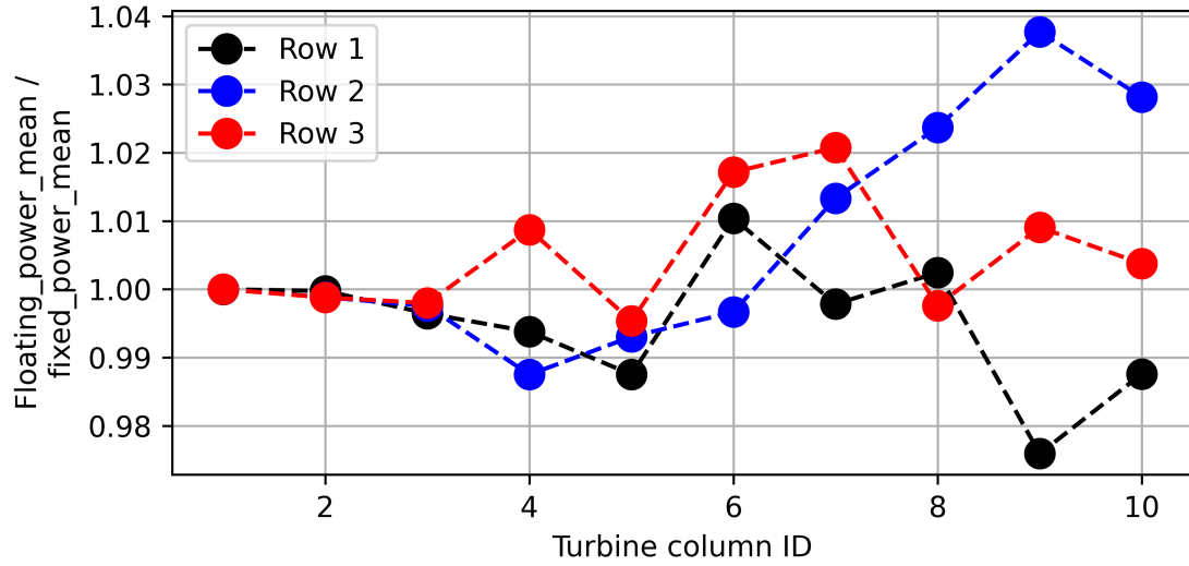
Figure 8. Plot of time-averaged (between 4 and 8 hours) power generation, ratio of Moving/Ocean to Fixed condition simulations. TI_{1.0} atmospheric conditions. Moving/Ocean simulations.
