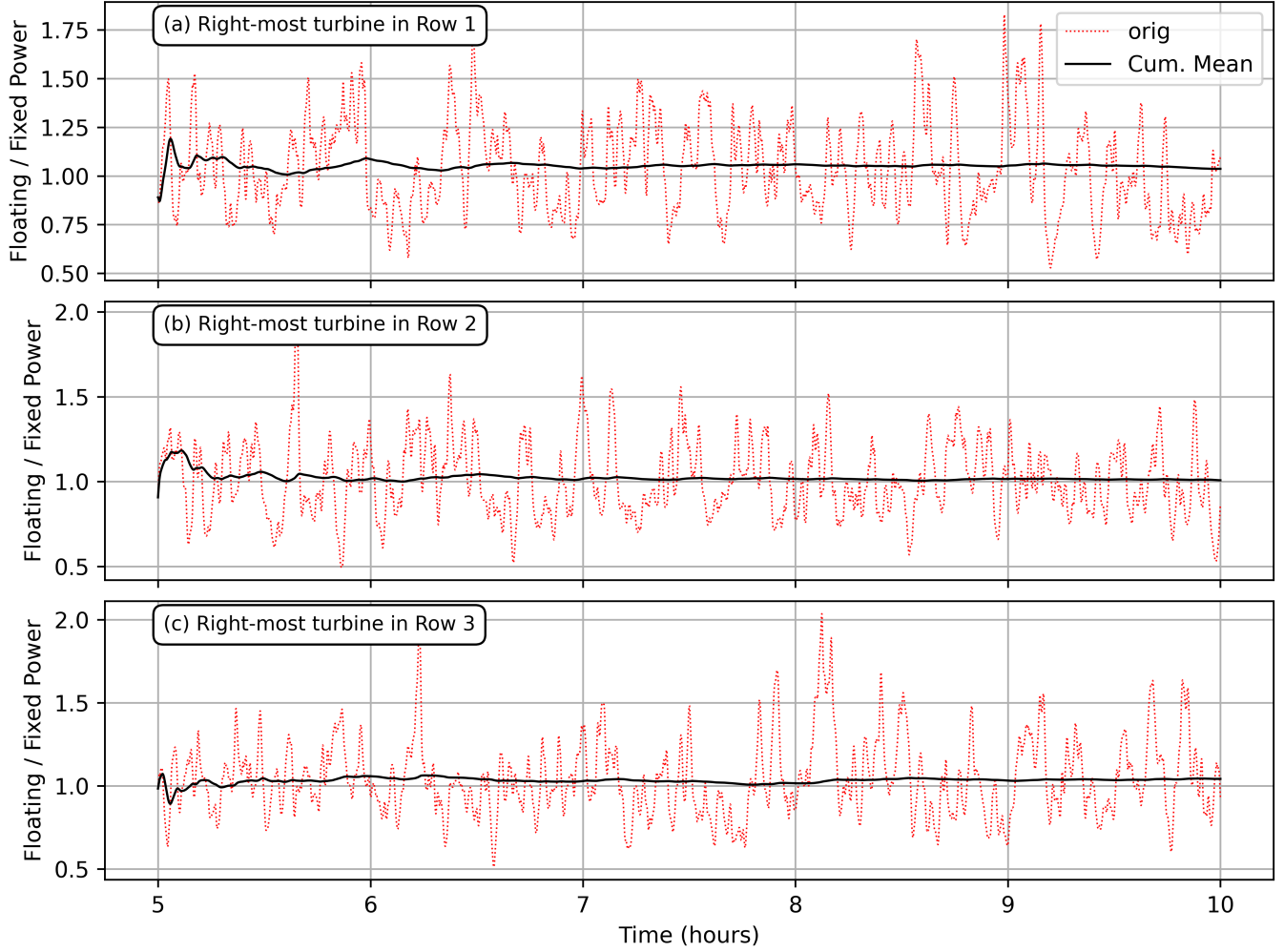
Figure 8. Floting-to-fixed relative power time series and its cumulative mean. Data taken from the right-most turbine (ID 10) in each row. The cummulative mean settles quickly, well before the span we take in averaging power outputs.
