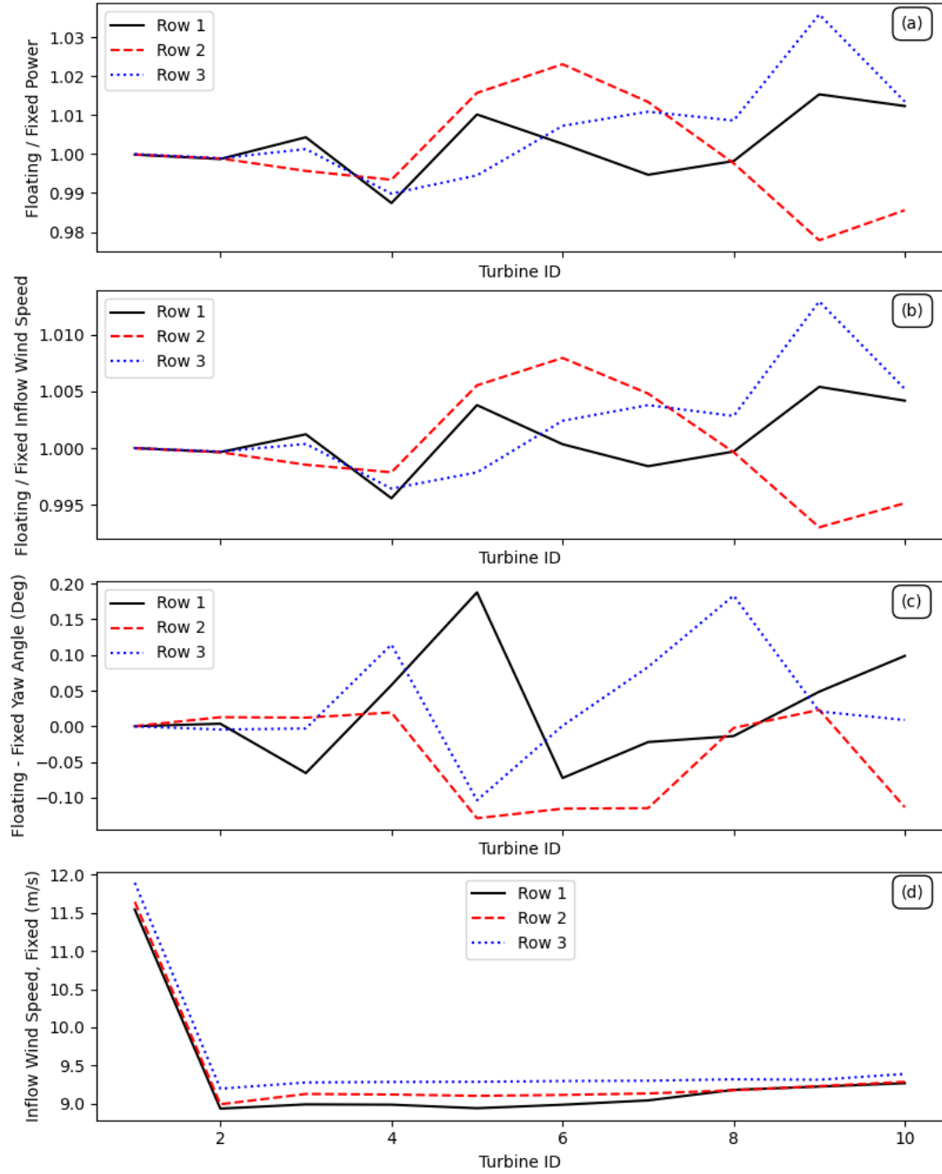
Figure 7. Plots of time-average over t \in [5, 10] hr and spatial average over z \in [90 - 63, 90 + 63] m for each individual turbine of (a) floating / fixed platform power production, (b) floating / fixed platform inflow wind speed normal to the disk, (c) floating - fixed platform yaw angle (degrees). Sub-figure (d) plots the fixed platform inflow wind speed for each turbine with the same averaging in space and time.
