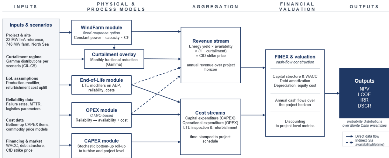
Figure 1. Schematic overview of the WINPACT module chain.
