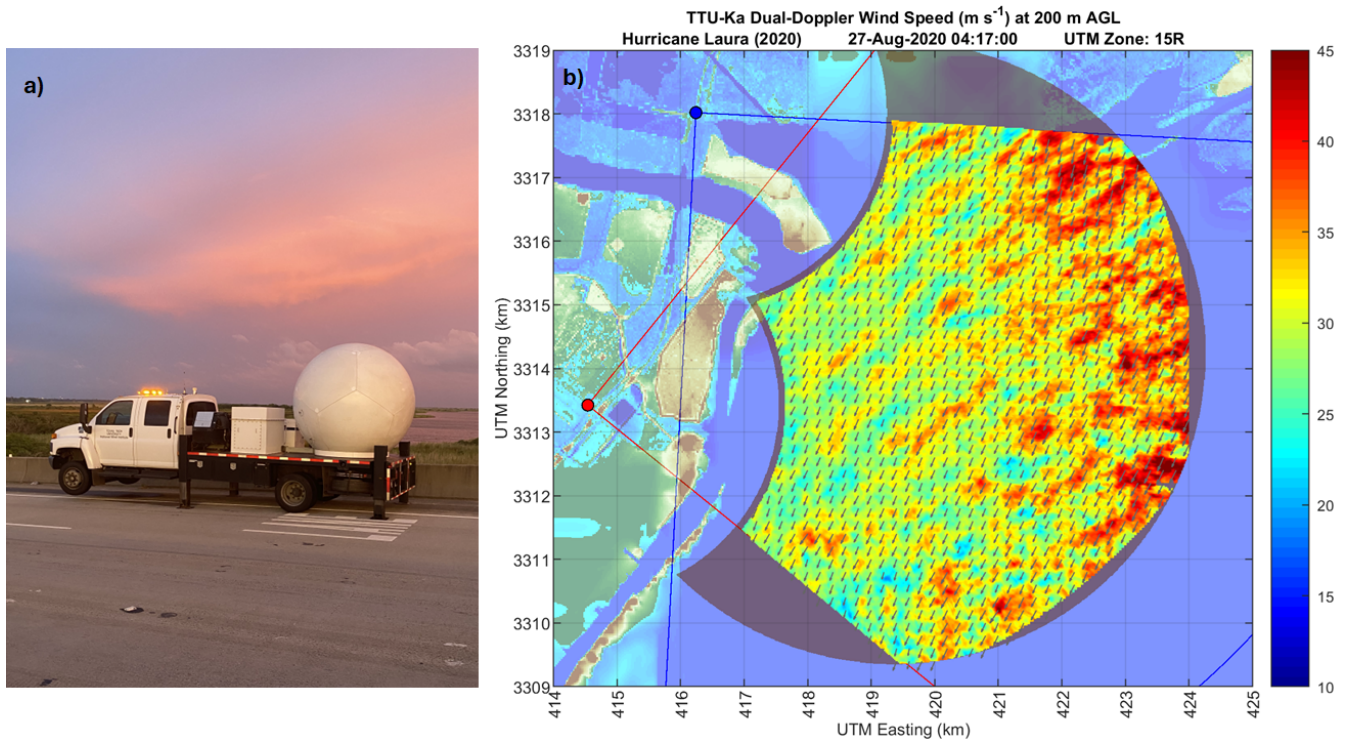
Figure 4. (a) TTU-Ka radar deployment during Hurricane Laura (2020) at Port Arthur, TX, and (b) a resulting snapshot dual-Doppler wind speed (m/s) map from 27-Aug-2020 04:17 UTC at 200 m AGL documenting detailed gust structure within Laura's wind field at the coastal interface.
