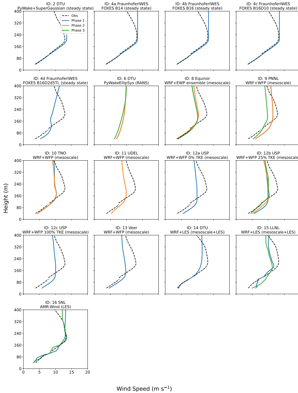
Figure 3. Modeled and observed wind speed profiles at Site A1 at 06:00 UTC on 24 August 2023. Profiles transition from profiling lidar data ( \leq 100 m a.g.l.) to scanning lidar measurements ( > 100 m a.g.l.); the discrepancy at this interface represents the inherent measurement uncertainty during instrument hand-off. Observations are matched to the time resolution (and average vs. instantaneous) of each model submission. Only models that submitted wind speed information at Site A1 are included in the plot. Meteodyn WT TM results are not included as the model is designed to provide long-term mean wind profile, not instantaneous snapshots.
