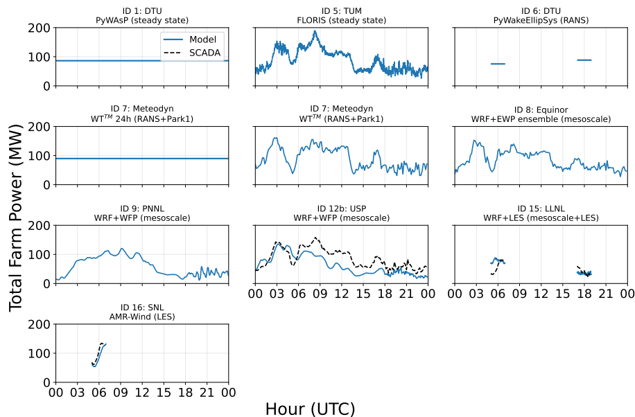
Figure 14. Time series of modeled and observed power at the King Plains wind farm on 24 August 2023 for each Phase 3 benchmark submission. Note that for submissions modeling only a subset of the turbines, the observed and modeled totals are calculated using only the corresponding turbines. Across all submissions, observed data are plotted at 10-minute resolution to increase readability. For the same goal, LES-modeled data are plotted using 2-minute instantaneous values.
