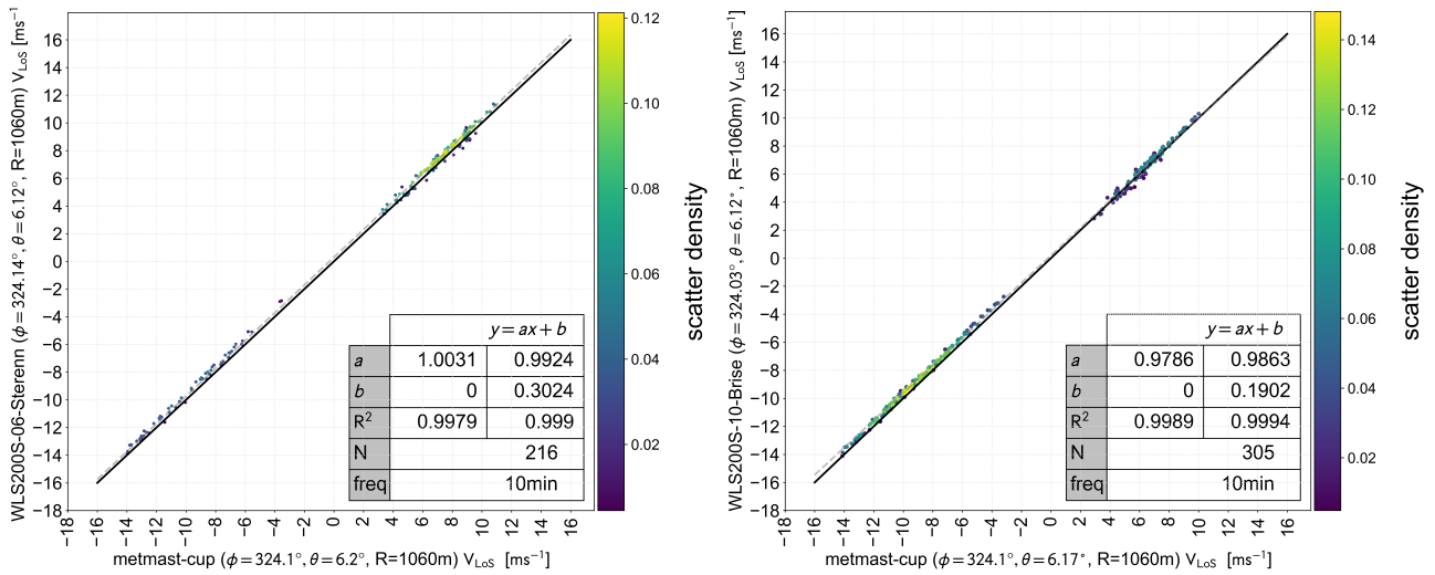
Figure 7. Regression analysis of the scanning lidar systems during the pre-calibration test against the metmast-met-mast cup anemometer for the different-models-WindScanner systems – left: Sterenn; right: Brise. Only wind direction from \pm 40^\circ of the line-of-sight direction and corresponding angles of 180^\circ apart have been kept for the analysis. Results of one and two-parameter fit are given in the table.
