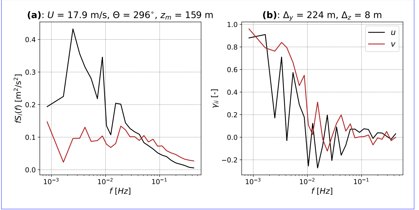
Figure 17. An example of auto-spectra and lateral coherence calculated from the lidar measurements over a period of 2 h with a mean wind speed of 17.9 m/s, mean wind direction of 296° and at a height of 159 m
