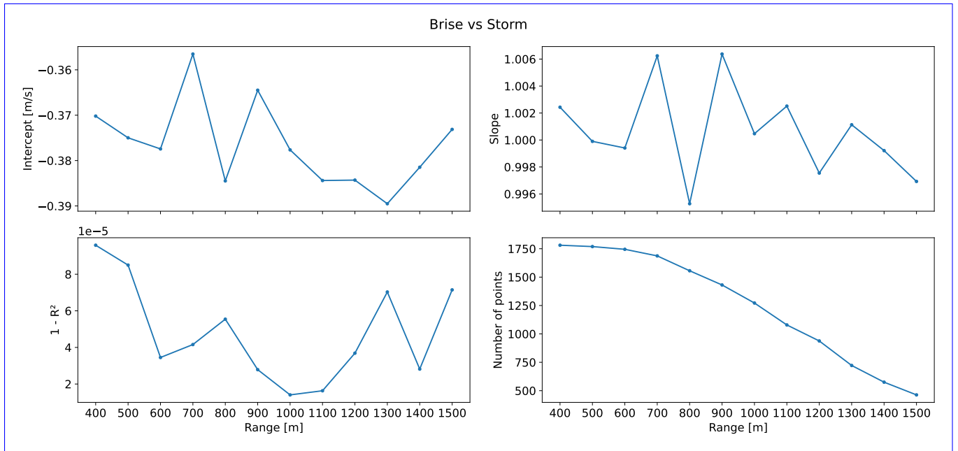
Figure 12. Linear fit parameters of post-campaign LOS speed inter-comparison between Brise and Storm across all ranges indicating good agreement between the two systems.
