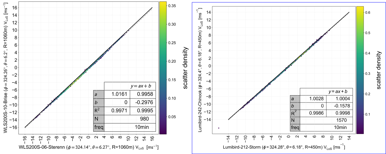
Figure 6. Regression analysis of the two pairs of scanning lidar systems during the pre-calibration test – left: WindScanner system with the range of comparison roughly at the met-mast ; right: Streamline/Lumibird system -The with the range of comparison is roughly at 450 m as the met-mast distance could rarely be reached. Results of one and two-parameter fit are given in the table.
