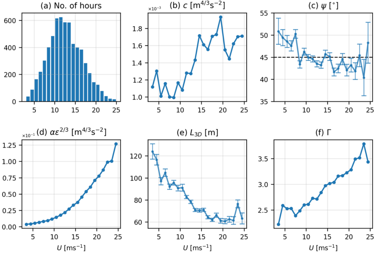
Figure 4. (a) The number of hours representing neutral atmospheric conditions at FINO1 at 81.5 m above sea level in 2007-2008 ( Total no. of hours = 6226 ). The data is divided into 1 \text{ ms}^{-1} bins from cut-in to cut-out wind speeds (3 to 25 \text{ ms}^{-1} ). (b) The scaling parameter c of the low-frequency turbulence model is obtained from fitting the spectra. (c) The mean anisotropy parameter \psi was obtained for the low-frequency wind fluctuations. (d), (e) and (f) represent the three Mann turbulence model parameters: \alpha\epsilon^{2/3} , L_{3D} , and \Gamma , respectively, obtained from spectral fitting. Error bars in (c) and (e) represent the standard error of the mean.
