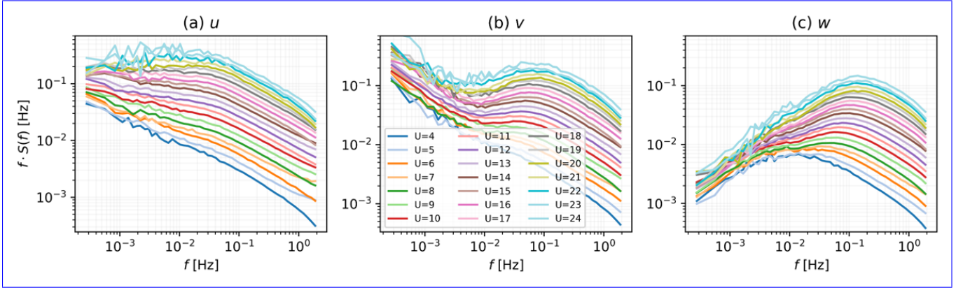
Figure 3. Mean spectra of hourly wind data as a function of frequency f for 1 \text{ ms}^{-1} wind speed bins (FINO1, z = 81 \text{ m} ) for the three wind components.
