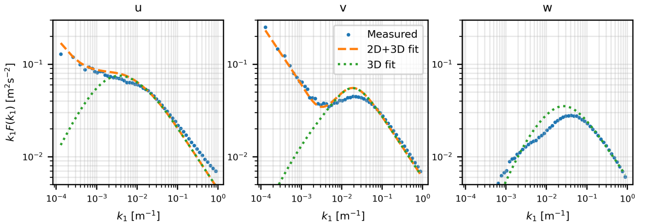
Figure 2. Wind velocity spectra measurements (blue dots) for \overline{U} = 13.5 \text{ ms}^{-1} at z = 81 \text{ m} from FINO1 under neutral atmospheric conditions. The 3D turbulence model (Mann spectral model) is fitted (green dotted lines) as well as the 2D+3D turbulence model (orange dashed lines) for u and v components
