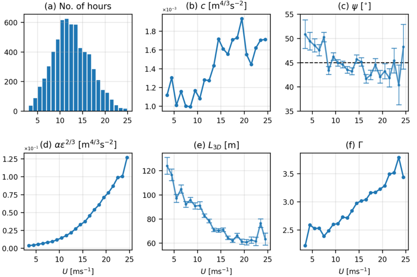
Figure 4. (a) The number of hours representing neutral atmospheric conditions at FINO1 at 81.5 m above sea level in 2007-2008 (Total no. of hours = 6226). The data is divided into 1 ms -1 bins from cut-in to cut-out wind speeds (3 to 25 ms -1 ). (b) The scaling parameter c of the low-frequency turbulence model is obtained from fitting the spectra. (c) The mean anisotropy parameter \psi was obtained for the low-frequency wind fluctuations. (d), (e) and (f) represent the three Mann turbulence model parameters: \alpha \epsilon^{2/3} , L_{3D} , and \Gamma , respectively, obtained from spectral fitting. Error bars in (c) and (e) represent the standard error of the mean.
