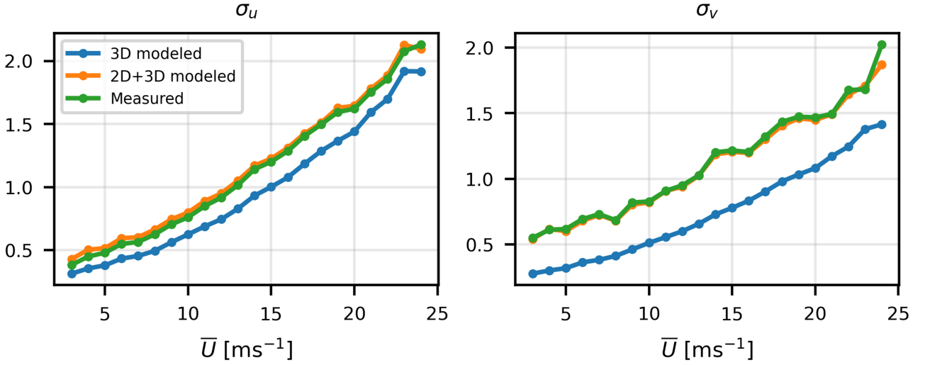
Figure 5. Modeled standard deviations \sigma_u and \sigma_v compared to the measured values for 2D+3D model and 3D model
