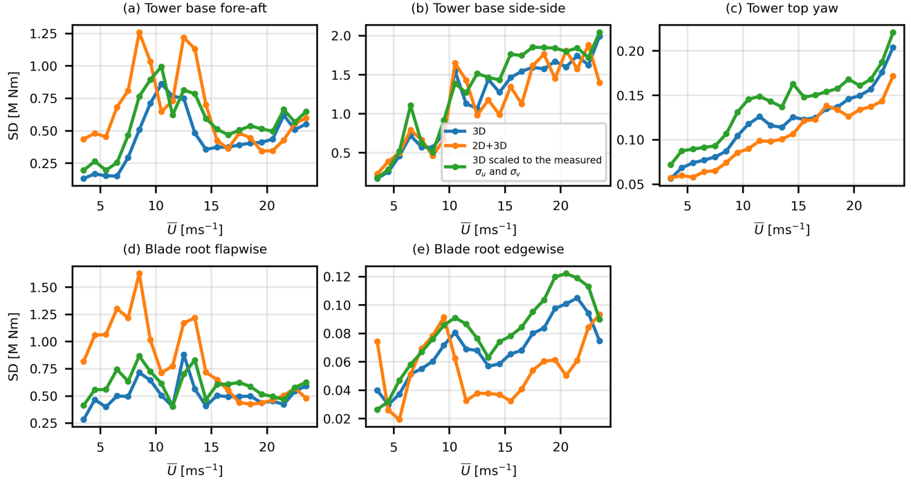
Figure 7. Same as Fig. 6 but the values represent the standard deviation
