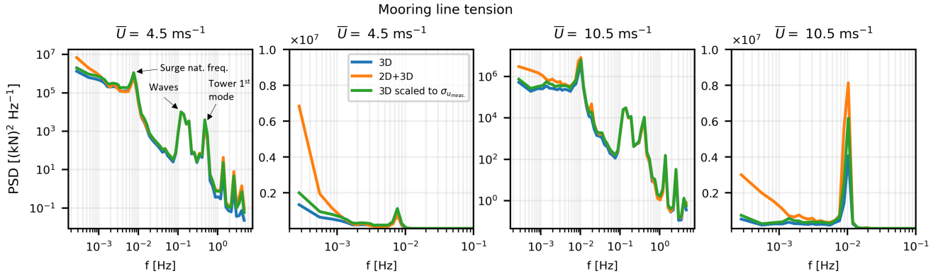
Figure 15. The response of the mooring line tension to different wind fields. These responses are shown for two wind speeds, i.e., 4.5 and 10.5 \text{ ms}^{-1} . The first and third columns represent the full frequency range on a log-log plot, while the second and fourth columns zoom into the low frequencies. Peaks corresponding to surge, waves, and tower motion are also indicated
