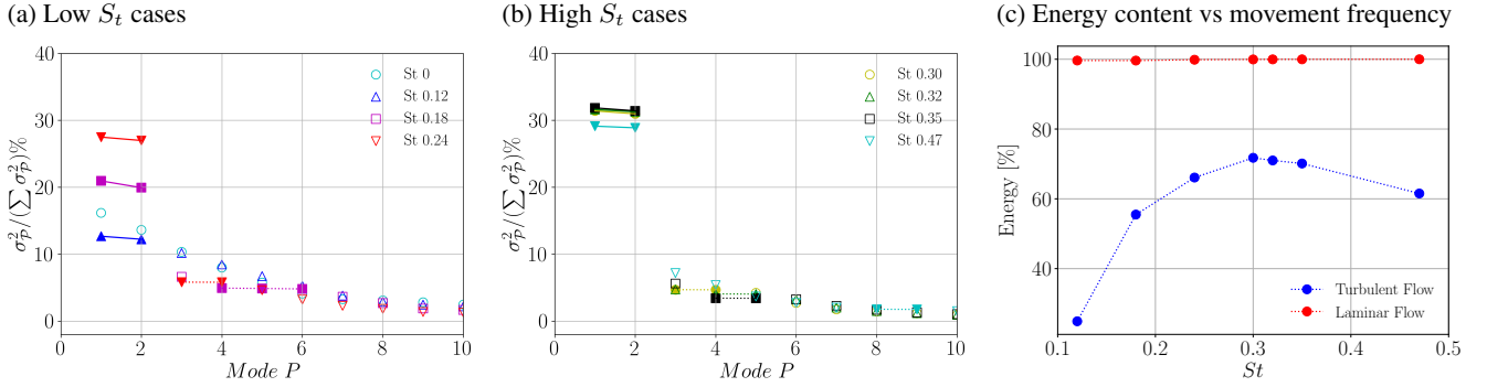
Figure 13. Energy content per mode in Low and High St values (a and b) and corresponding to the combined contribution of all modes associated with the vortex ring structure (c) as a function of the St number, under low-turbulence flow. In the first two plots, the filled markers connected by a dashed line indicate mode pairing corresponding to the surge frequency, while harmonics are connected with dotted lines.
