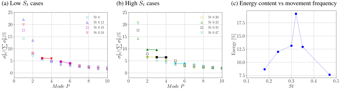
Figure 17. Energy content per mode in Low and High St values (a and b) and corresponding to the combined contribution of the two modes associated with the vortex ring structure (c) as a function of the St number, under ABL flow. In the first two plots, the filled markers connected by a dashed line indicate mode pairing.
