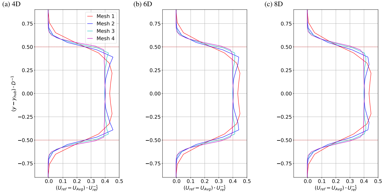
Figure 3. Average velocity deficit rev results for the mesh convergence study under laminar uniform flow at 4D, 6D and 8D rev downstream the AD.
