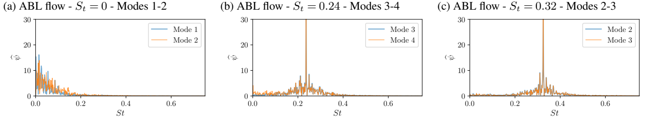
Figure 16. Fourier spectrum of the temporal modes \Psi_1(t) and \Psi_2(t) for S_t = 0 (a), modes \Psi_3(t) and \Psi_4(t) for S_t = 0.24 (b) and modes \Psi_2(t) and \Psi_3(t) for S_t = 0.32 (c), under ABL flow. Modes 1 and 2 for S_t = 0.24 and modes 1 and 4 for S_t = 0.32 have similar spectra as the ones displayed by modes 1 and 2 in S_t = 0 .
