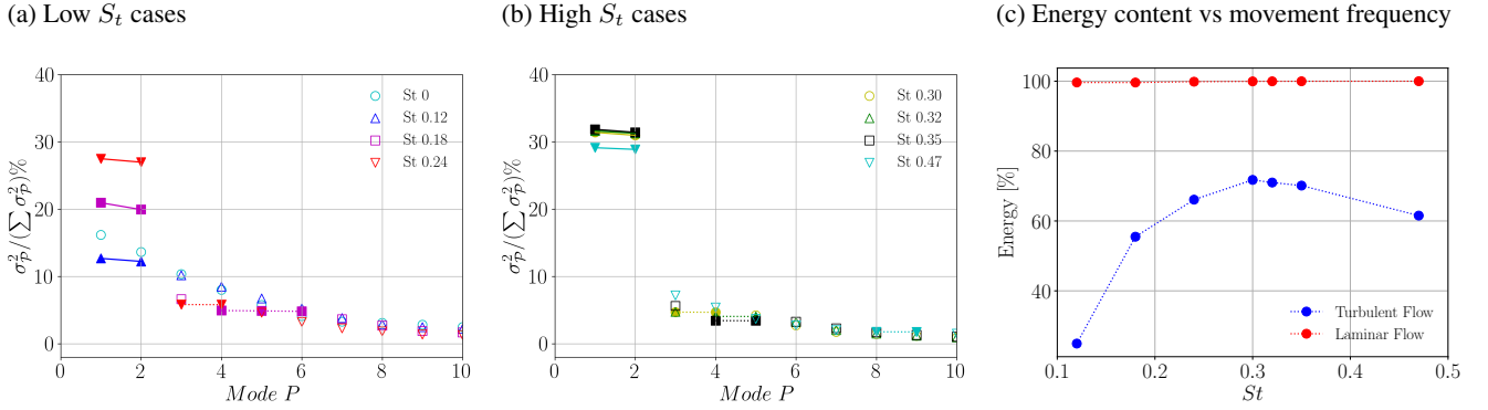
Figure 13. Energy content per mode in Low and High St values (a and b) and corresponding to the combined contribution of all modes associated with the vortex ring structure (c) as a function of the St number, under low-turbulence flow. In the first two plots, the filled markers connected by a dashed line indicate mode pairing corresponding to the surge frequency, while harmonics are connected with dotted lines.
