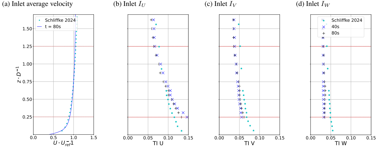
Figure 5. Inlet flow average velocity (a) and TI profiles for the three velocity components (b, c and d) after mesh refinement. All profiles are zoomed in the refined region and compared with experimental values from Schliffke et al. (2024). The dotted red lines delimit the height of the porous disk.
