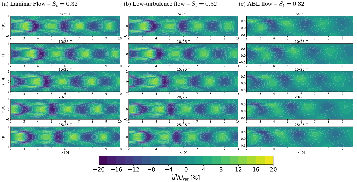
Figure 21. Phase averaged streamwise velocity fluctuations for laminar flow (a), low-turbulence flow (b) and ABL flow (c). Out of the 25 averaged planes within the surge period, 5 planes uniformly distributed are shown.
