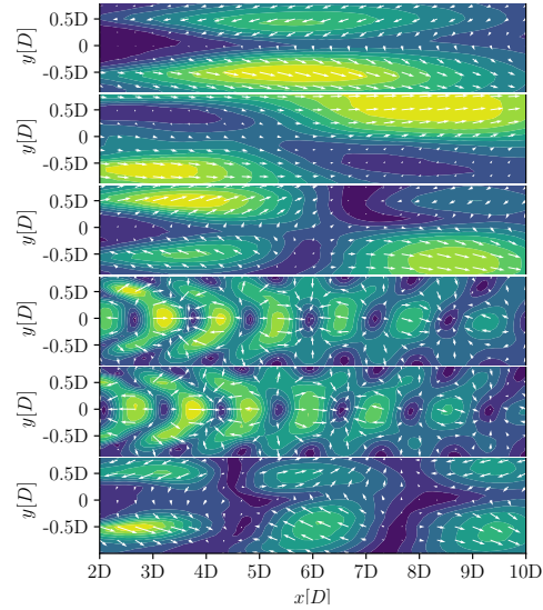
(b) ABL flow - S_t = 0.32
