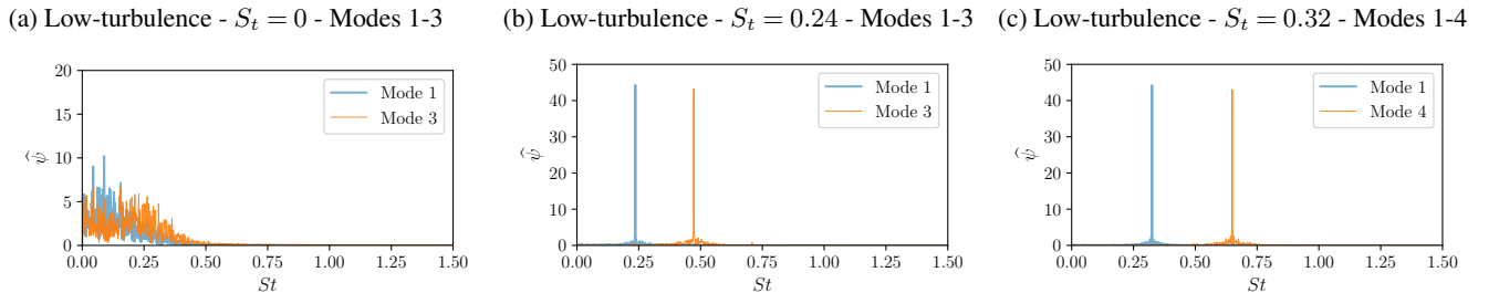
Figure 12. Fourier spectrum of the temporal modes \Psi_1(t) and \Psi_3(t) for S_t = 0 (a), \Psi_1(t) and \Psi_3(t) for S_t = 0.24 (b) and \Psi_1(t) and \Psi_4(t) for S_t = 0.32 (c), under low-turbulence flow.
