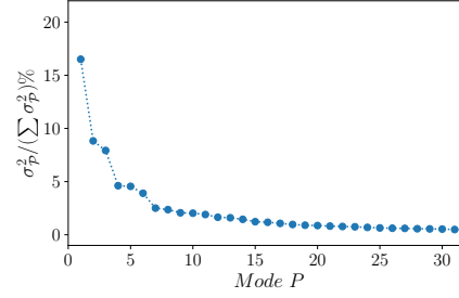
Figure 18. Energy distribution across modes resulting from POD analysis applied to a horizontal plane on cases with S_t = 0.32 under low-turbulence flow (a) and ABL flow (b).
