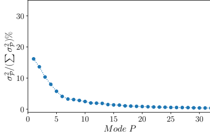
Figure 10. Energy distribution across modes for S_t = 0 (a), S_t = 0.24 (b) and S_t = 0.32 (c), under low-turbulence flow.
