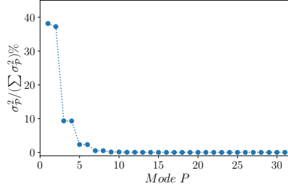
Figure 7. Energy distribution across modes for S_t = 0 (a), S_t = 0.24 (b) and S_t = 0.32 (c), under laminar flow.
