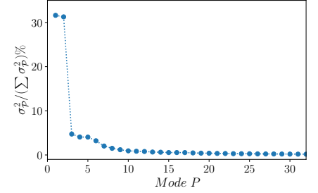
Figure 10. Energy distribution across modes for S_t = 0 (a), S_t = 0.24 (b) and S_t = 0.32 (c), under low-turbulence flow.
