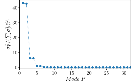
Figure 7. Energy distribution across modes for S_t = 0 (a), S_t = 0.24 (b) and S_t = 0.32 (c), under laminar flow.
