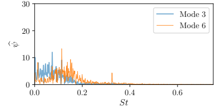
Figure 20. Fourier spectrum of the temporal modes \Psi_1(t) and \Psi_2(t) (a), \Psi_4(t) and \Psi_5(t) (b) and \Psi_3(t) and \Psi_6(t) (c) for S_t = 0.32 under ABL flow.
