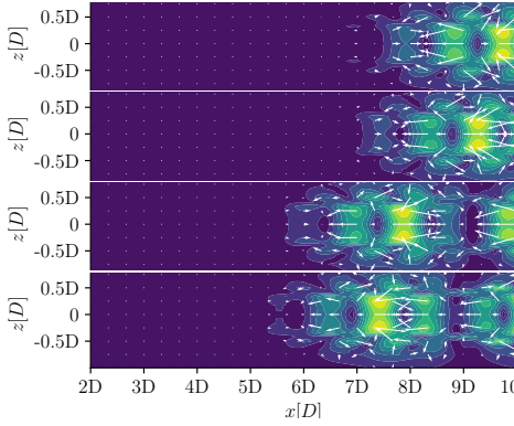
(a) Laminar flow - S_t = 0
