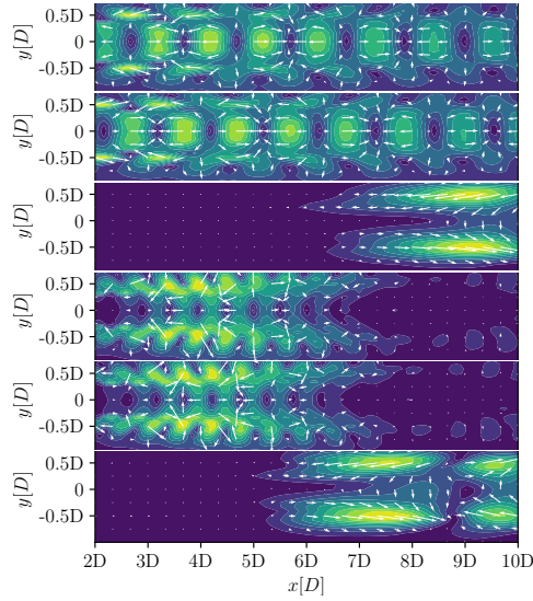
(a) Turbulent flow - S_t = 0.32
