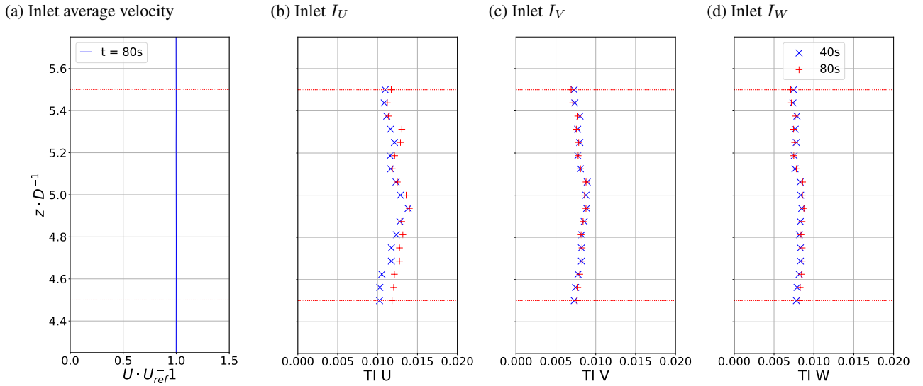
Figure 4. Inlet flow average velocity (a) and TI profiles for the three velocity components (b, c and d) after mesh refinement for low-turbulence flow. All profiles are zoomed in the refined region. The dotted red lines delimit the height of the porous disk.
