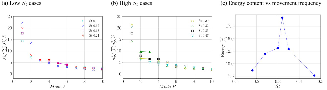
Figure 17. Energy content per mode in Low and High St values (a and b) and corresponding to the combined contribution of the two modes associated with the vortex ring structure (c) as a function of the St number, under ABL flow. In the first two plots, the filled markers connected by a dashed line indicate mode pairing.
