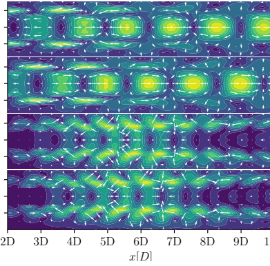
(b) Laminar flow - S_t = 0.24
