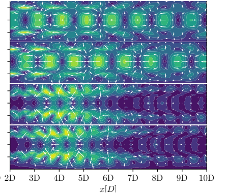
(c) Laminar flow - S_t = 0.32
