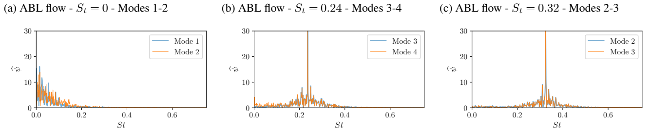
Figure 16. Fourier spectrum of the temporal modes \Psi_1(t) and \Psi_2(t) for S_t = 0 (a), modes \Psi_3(t) and \Psi_4(t) for S_t = 0.24 (b) and modes \Psi_2(t) and \Psi_3(t) for S_t = 0.32 (c), under ABL flow. Modes 1 and 2 for S_t = 0.24 and modes 1 and 4 for S_t = 0.32 have similar spectra as the ones displayed by modes 1 and 2 in S_t = 0 .
