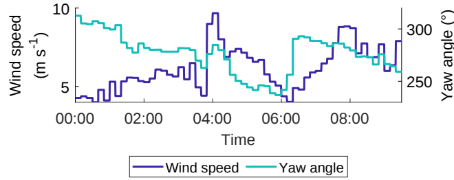
Figure 17. 10 minute mean values of the yaw angle and wind speed during the considered period.
