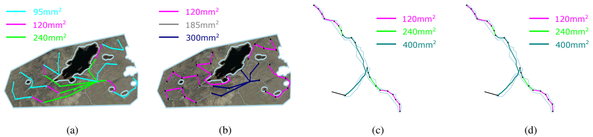
Figure 8. Onshore array results showing integrated and sequential CSS solutions respectively for each case: (a,b) Bhlaraidh [GB-SCT] , (c,d) Coromuel [MX]
