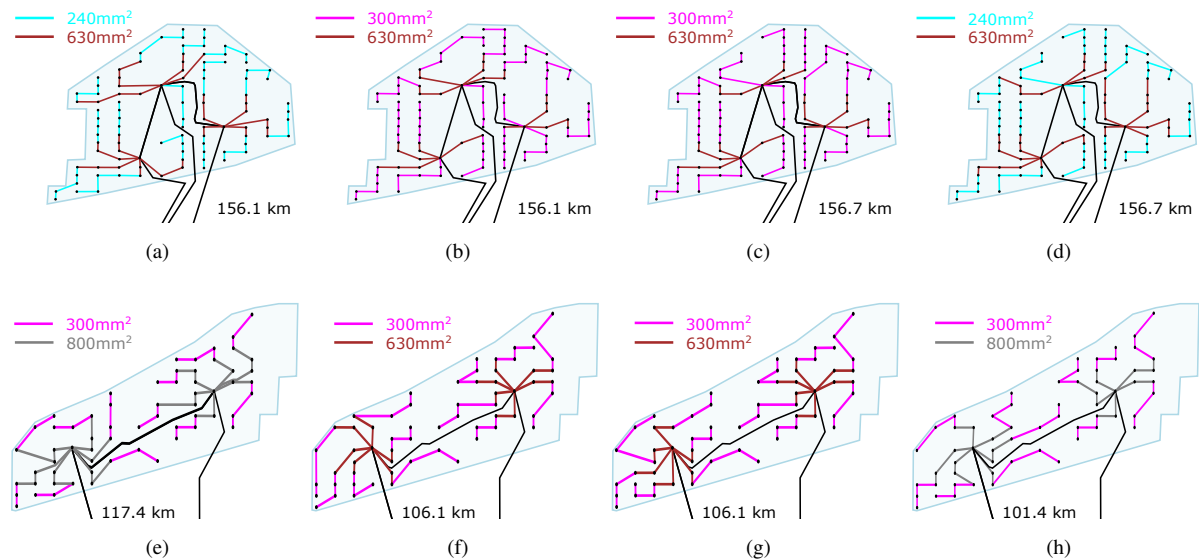
Figure 9. Project comparison for Moray East (a–d) and Moray West (e–h) [GB-SCT]: actual reported layouts and layouts obtained using the integrated, linear sequential, and non-linear sequential methodologies.
