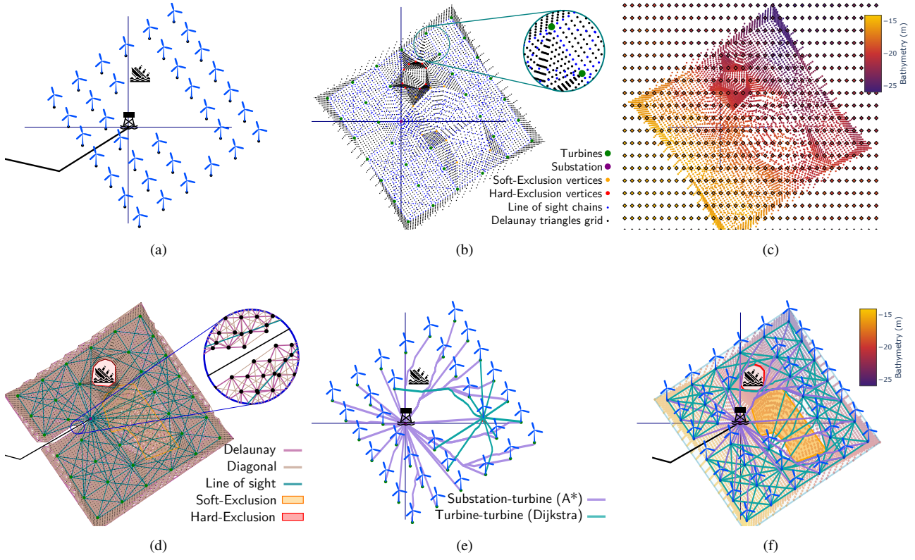
Figure 1. Graph edge preparation: (a) Turbine group, (b) Densified grid, (c) Elevation overlay, (d) Densified graph, (e) Inter-paths, (f) Final graph.
