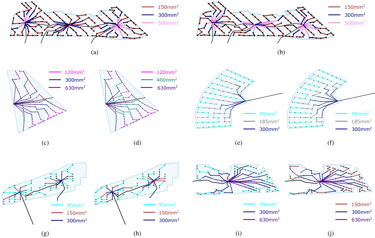
Figure 7. Offshore array results showing integrated and sequential CSS solutions respectively for each case: (a,b) Hornsea I [GB-ENG], (c,d) Anholt [DK], (e,f) Horns Rev 2 [DK], (g,h) Moray West [GB-SCT], (i,j) Seagreen [GB-SCT]
