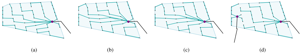
Figure 4. Baltic Eagle [DE] array results: solutions from model parameters set to (a) Core formulation, (b) minimum number of turbines per string, (c) allowing bifurcations, and (d) irregular substation capacities.
