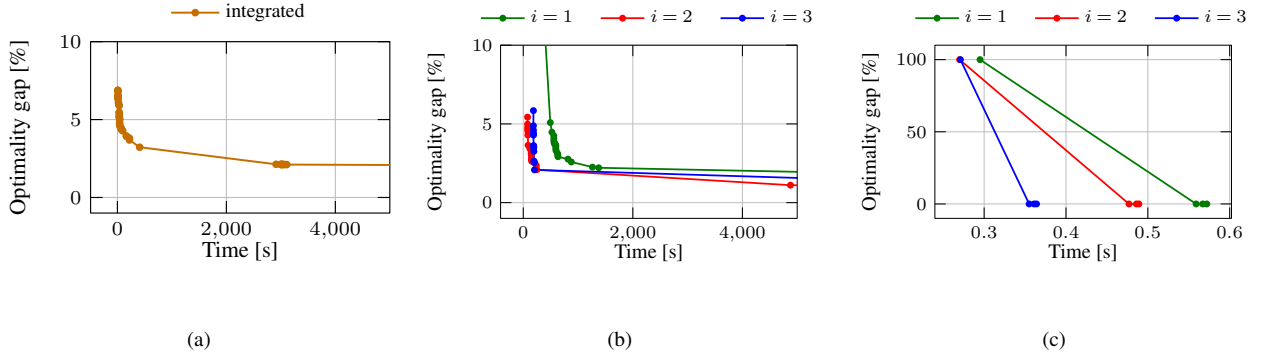
Figure 10. Solver progress for the case HornSea I [GB-ENG] : (a) Integrated CSS-MILP, (b) Sequential: minimum path connection with minimum turbines and determining substation connections and (c) Sequential: CSS
