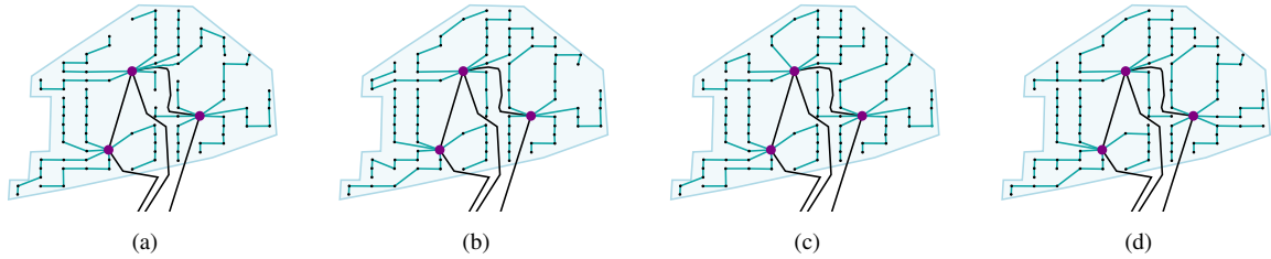
Figure 5. Moray East [GB-SCT] array results: solutions from model parameters set to (a) Core formulation, (b) determining substation connections, (c) minimum number of turbines per string and determining substation connection , and (d) allowing bifurcations.
