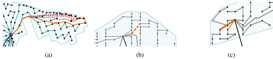
Figure 11. Onshore array results showing integrated and sequential CSS solutions respectively for each case: (a) Section of Hornsea II connectivity, (b) Moray East Delaunay and diagonals restriction, (c) Moray West Static Crossings
