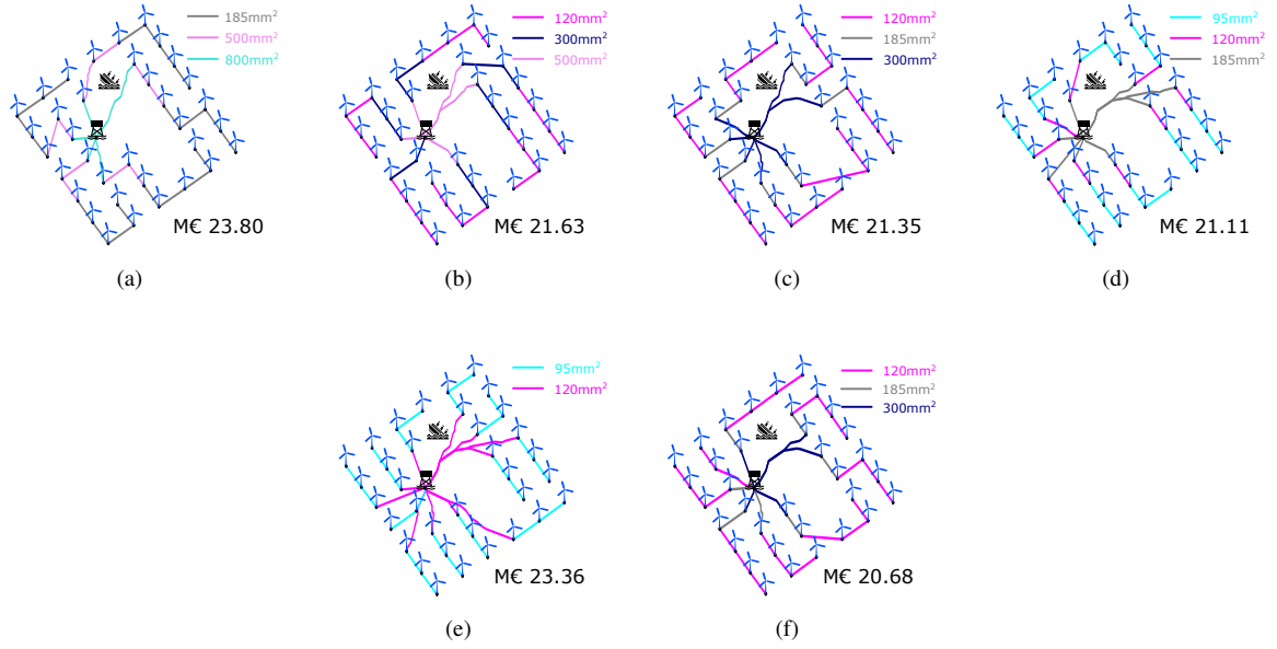
Figure 6. Westermost Rough [GB-ENG] array results: iterative solutions from (a) iteration 1 to (e) iteration 5, and (f) the integrated MILP formulation.
