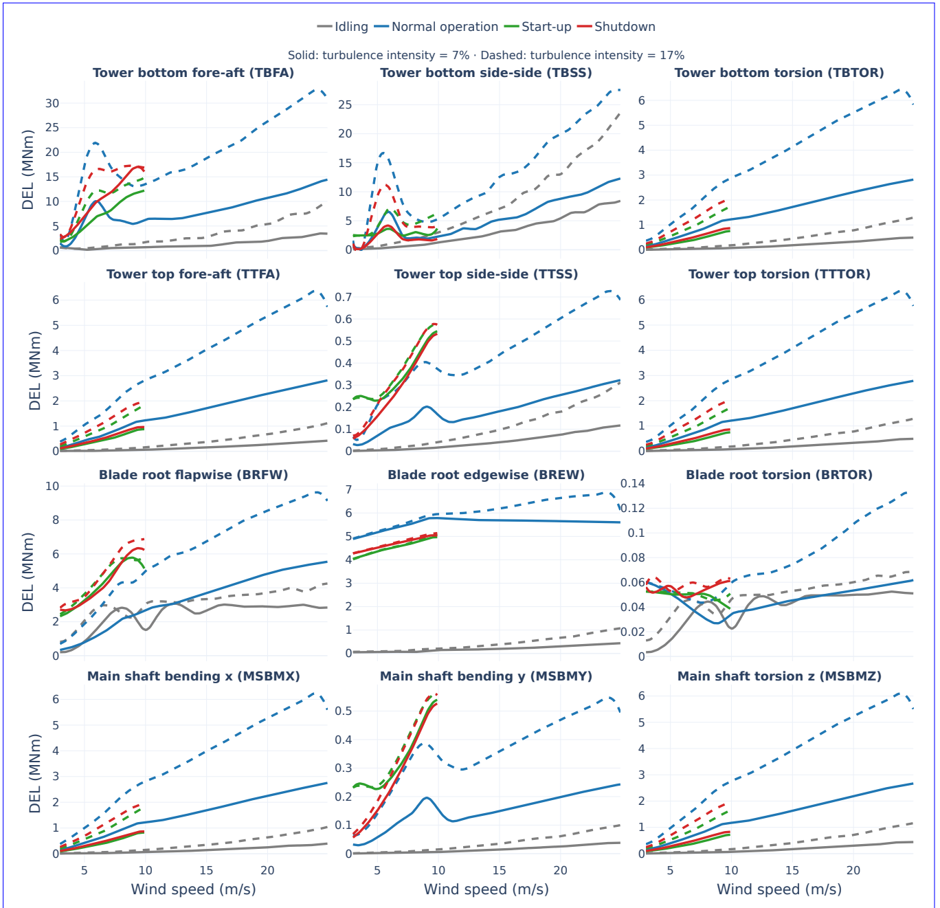
Figure 5. Parametric sweeps of selected surrogate-predicted DEL DELs for all considered structural load channels as a function functions of wind speed for constant turbulence intensity at turbulence intensity levels of 7% (solid lines) and 17% (dashed lines), shown for each operational mode.
