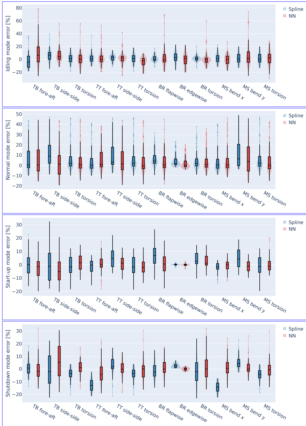
Figure B1. Comparison of surrogate model accuracy on the independent test set for spline interpolation and neural networks. Violin plots summarize the distribution of signed percentage errors across channels for each operational mode. Overlapping box plots show mean along with 25th and 75th percentiles. The 2% of the distribution tails have been trimmed to improve readability.
