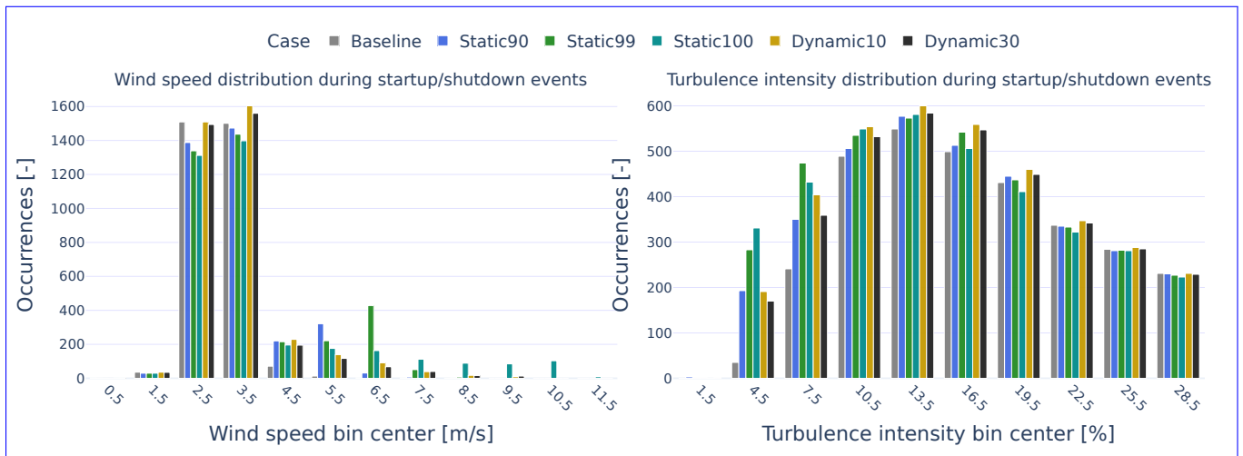
Figure 12. Histograms of ambient wind speed (left) and turbulence intensity (right) at the times of start-up/shutdown events, aggregated over the full evaluation period for all evaluated cases.
