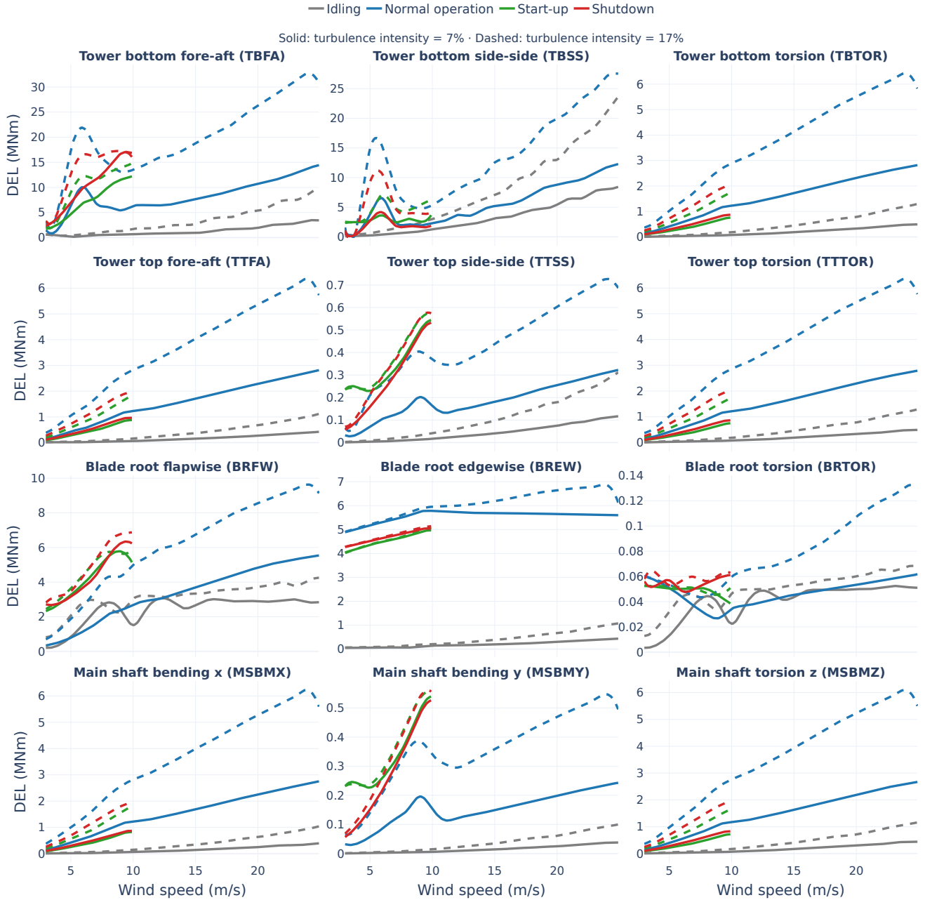
Figure 5. Parametric sweeps of surrogate-predicted DELs for all considered structural load channels as functions of wind speed at turbulence-intensity levels of 7 % (solid lines) and 17 % (dashed lines), shown for each operational mode.
