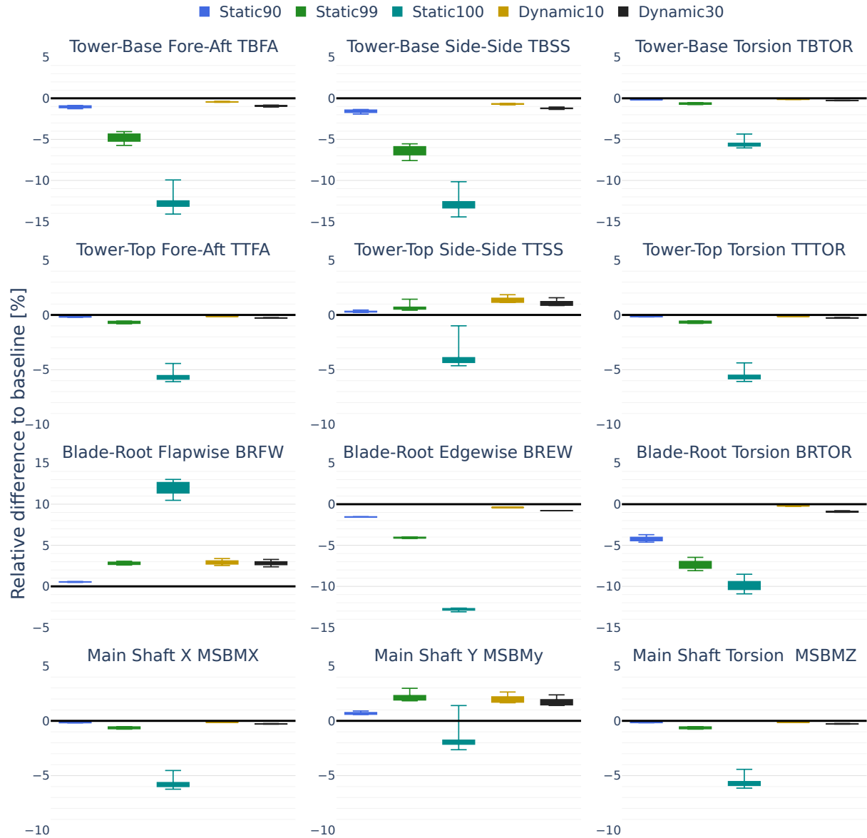
Figure 11. Relative differences in cumulative fatigue damage with respect to the baseline case for the full evaluation period. Each subplot corresponds to one load channel, and box plots summarize the distribution across turbines for the evaluated strategies. The box spans the 25th to 75th percentiles, and the whiskers denote the minimum and maximum values.
