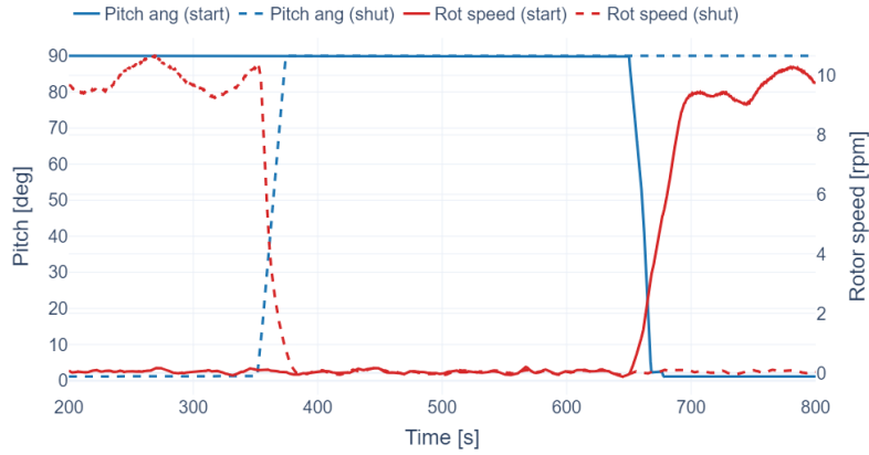
Figure 3. Illustrative aeroelastic time series of pitch angle and rotor speed for start-up and shutdown simulations, showing the imposed structure within the 10-minute evaluation interval and the timing of the maneuver relative to normal-operation and idling segments.
