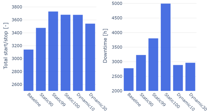
Figure 10. Operational impact of the evaluated strategies over the full two years period. Left: total number of start-up and shutdown events. Right: total downtime in hours, defined as the cumulative time spent in shutdown, idling, and start-up modes.
