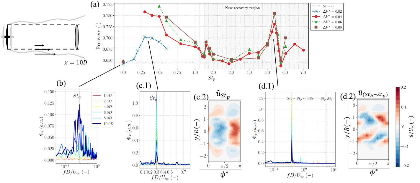
Figure 2. (a) Extended recovery curve, i.e recovery against St at x = 10D for \Delta V^* \in [0.02, 0.08] at TSR = 9 , St_b = f_b D/U_\infty \approx 5.75 and C_T = 0.8 . Power spectra of the wind speed fluctuation in the shear layer of the wake at y = R and x \in [1, 10]D for St_p = 0 (b), St_p = 0.3 (c.1) and St_p = 5.39 (d.1). Phase-averaged of wind speed coherent fluctuations, \tilde{u}/U_\infty at x = 4D at St_p = 0.3 (c.2) and St_b - St_p \sim 0.35 (d.2). Laminar inflow with TI_\infty = 0.3\% (no grid).
