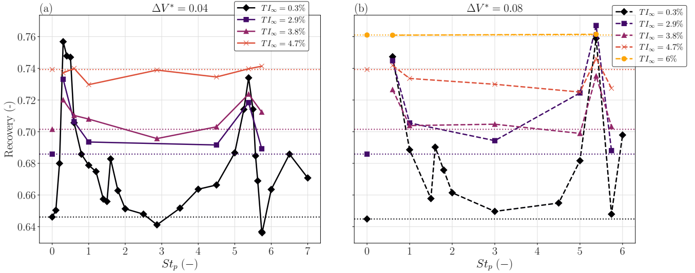
Figure 4. Recovery ( R ) against reduced frequency St_p , and two \Delta V^* , for different levels of turbulence intensity up to 6% (with active grid). TSR = 9 , St_b = f_b D/U_\infty \approx 5.75 and C_T = 0.80 .
