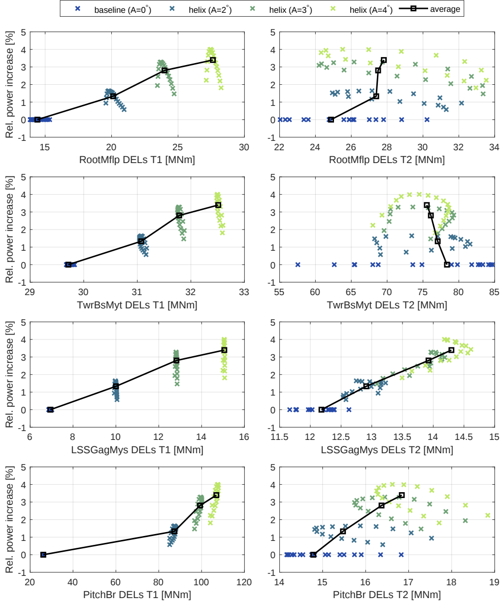
Figure 12. Tradeoff between the relative power increase ( (P_{WEFC}/P_{BL} - 1) \times 100\% ) and loads of a two-turbine array as predicted by the surrogate model. The left column shows the loads of T1, and the right column those of T2. The average relation between power gain and loads is determined by weighting the estimates with a Gaussian wind direction distribution.
