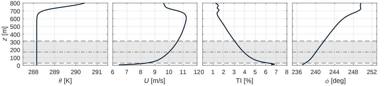
Figure 1. Average profiles of temperature ( \theta ) , wind speed ( U ), turbulence intensity ( I ) and wind veer ( \phi ) over height ( z ) for one the precursor simulations in AMR-Wind. The dash-dotted line indicates the turbine hub-height, while the shaded areas indicate the height spanned by the wind turbine rotor.
