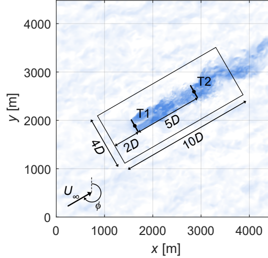
Figure 2. Schematic of the-a simulation setup in AMR-Wind. The simulation domain has dimensions 15.7 D \times 15.7 D \times 4.5 D . A single mesh refinement ( 4 D \times 10 D \times 2.1 D ) is indicated by the rectangle enclosing the turbines. The two turbines are separated by a distance of 5 D . The flow is coming from the southwest direction of the simulation domain.
