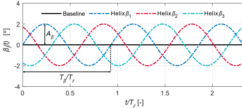
Figure 3. Example of the pitch reference signals ( \beta_i ) for the counterclockwise helix implementation. Time-The amplitude of the signals is indicated by A_\beta . The period of the pitch actuation is given by T_\beta = f_\beta^{-1} , normalized by the duration of one rotor rotation period t_r = f_r^{-1} T_r = f_r^{-1} .
