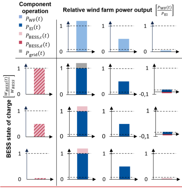
Figure 2: Overview of power flows of HPP components for timestep in the assumed determined operation strategy- for a timestep depending on the relative WF power output (top row) and the BESS state of charge (left column).
