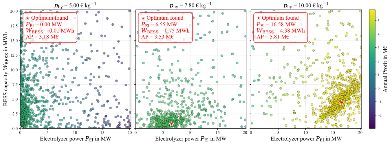
760 Figure 7: AnnualDesign space exploration of annual profit as function of electrolyzer rated power and rated BESS capacity over wind farm rated power via differential evolution for three different hydrogen prices.
