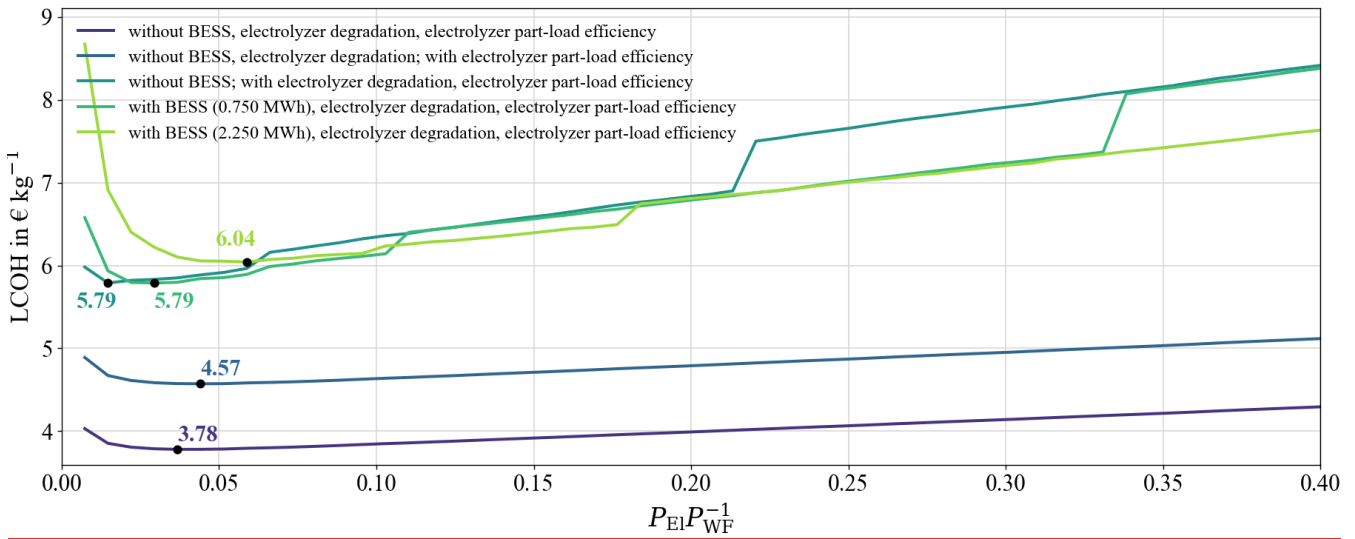
Figure 8: LCOH over the ratio of electrolyzer rated power to wind farm rated power for four different modelling modeling approaches and two different BESS sizes.
