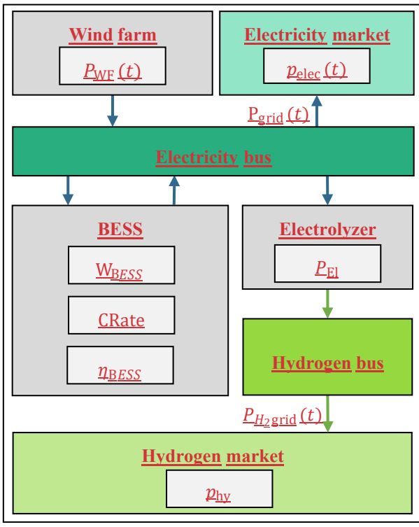
Figure 6: Schematic overview of the modelled modeled energy system for the operation optimization in oemof.
