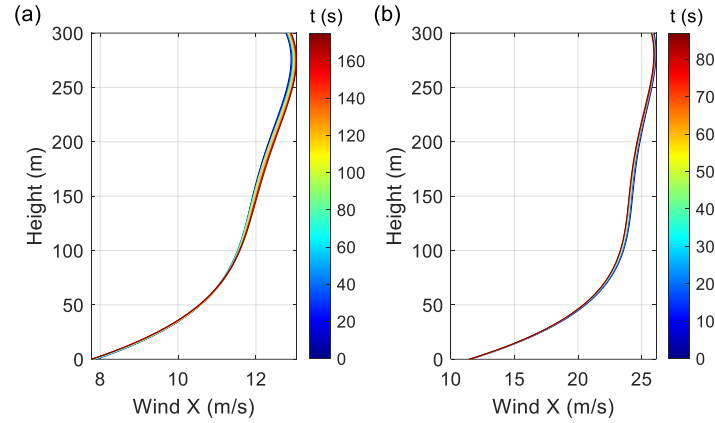
Figure 18. Medium (a) and high (b) wind fields implemented in the simulation based on LiDAR data.
