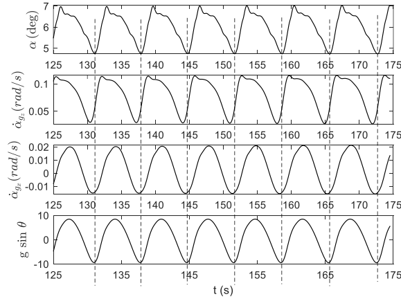
550 Figure 28. Potential feedback terms to cancel out the effect of gravity on \alpha oscillation.
