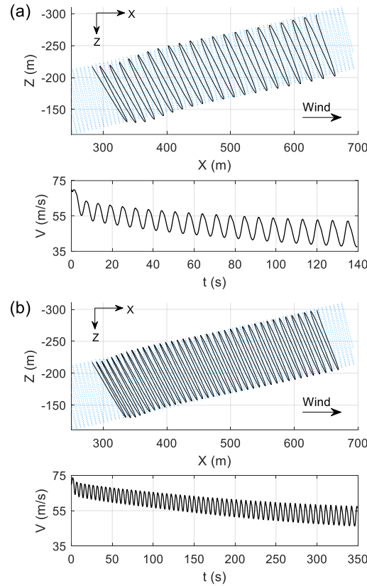
Figure 21. Reeling out at 2.5 m/s (a) and 1.0 m/s (b) winch speed, showing lower airspeed in (a) due to faster reel out.
