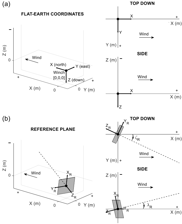
175 Figure 4. Two coordinate systems: Earth (a) and reference plane (b).
