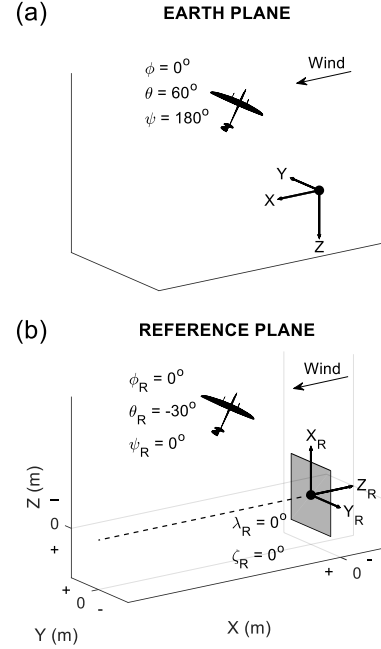
180 Figure 5. Illustrations of Euler angles on the Earth plane (a) and reference plane with \lambda_R = \zeta_R = 0^\circ (b).
