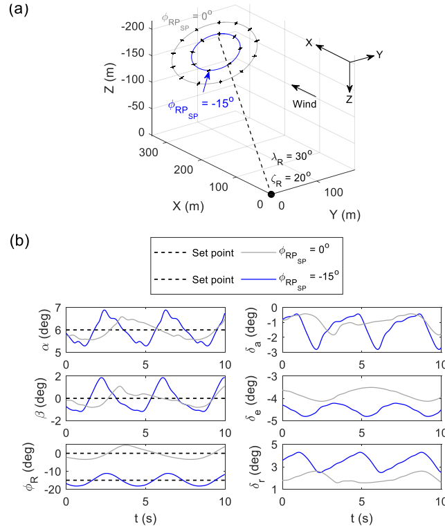
Figure 10. Closed-loop trajectories (a) and time histories (b) with different \phi_{RSP} . The kite is drawn true to scale at 0.5-second intervals.
