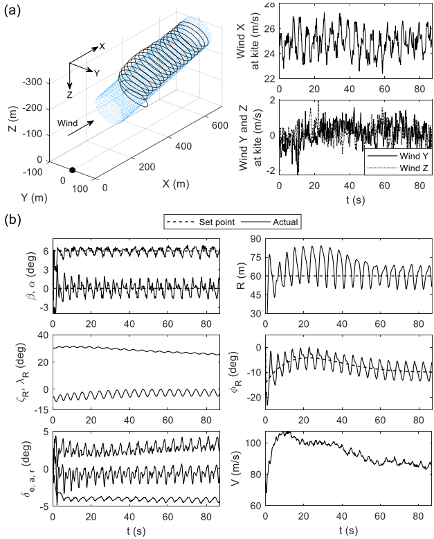
Figure 20. Reel out in high wind and high turbulence. The winch speed is kept constant at 4.0 m/s.
