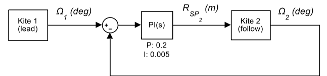
Figure 32. Phase synchronisation controller in the second kite.
