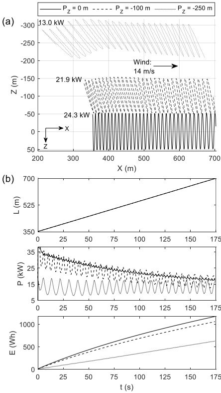
Figure 24. Different power production capacities at different heights due to cosine loss.
