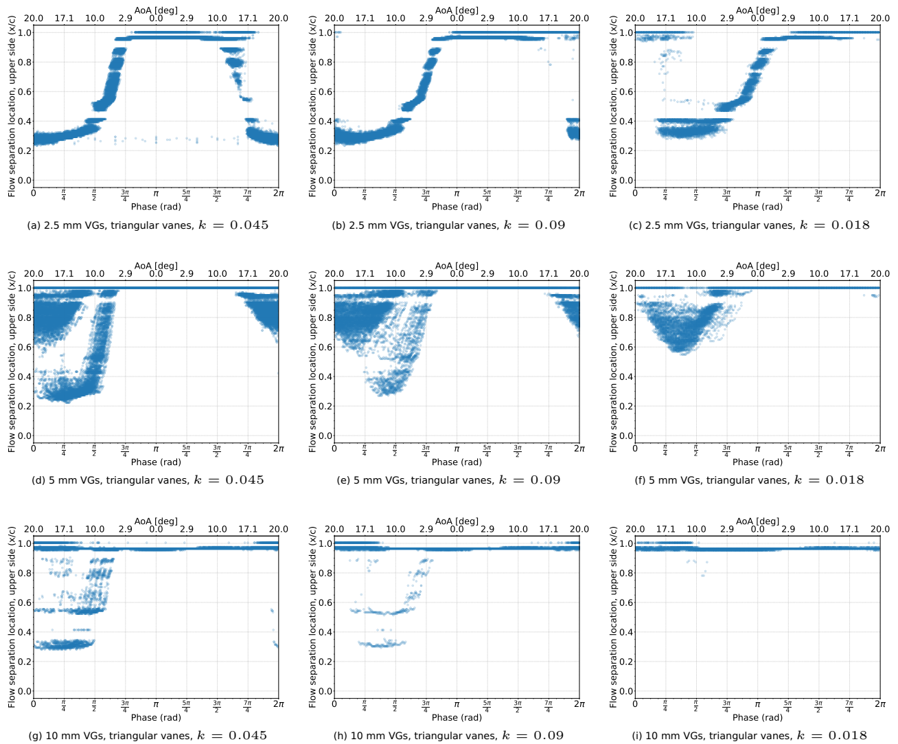
Figure 11. Flow separation location on the suction side over 150 pitching cycles of 10^\circ \pm 10^\circ when the airfoil is equipped with triangular vane VGs of three different vane sizes.
