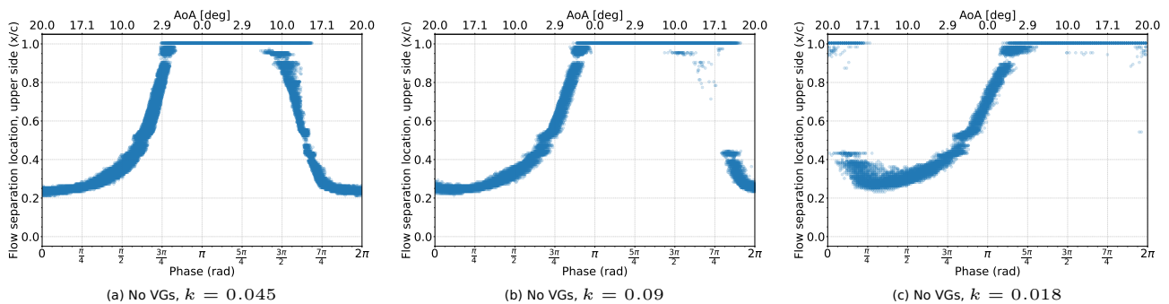
Figure 9. Flow separation location on the suction side over 150 pitching cycles of 10^\circ \pm 10^\circ in the absence of VGs.
