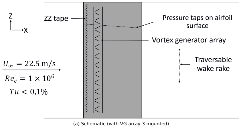
(a) Schematic (with VG array 3 mounted)
