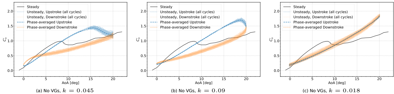
Figure 8. Normal force coefficient polars for the 10^\circ \pm 10^\circ pitching motion in absence of VGs.
