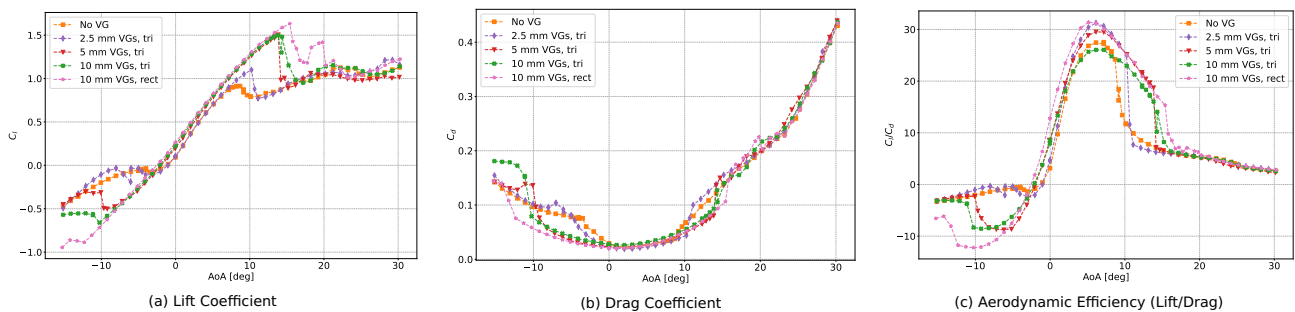
Figure 6. Comparing the stall delay, lift enhancement, drag penalty, and aerodynamic efficiency for different VG heights and shapes.
