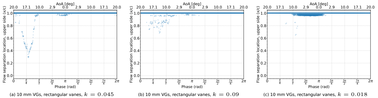
Figure 13. Flow separation location on the suction side over 150 pitching cycles of 10^\circ \pm 10^\circ angle of attack when the airfoil is equipped with rectangular vane VGs.
