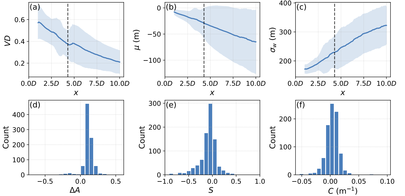
Figure 7. Mean (lines) and region of \pm 1 standard deviation (shades) of the velocity deficit VD (a), lateral wake center deflection \mu (b) and wake width \sigma_w (c) from 1 to 10 D downstream deduced from lidar data with 20 m range gate separation. Histograms of asymmetry \Delta A (d), vertical slope S (e) and vertical curl C (f) at 1 D . In (a)-(c) the vertical black dashed line indicates the location of OPUS2 at 4.3 D .
