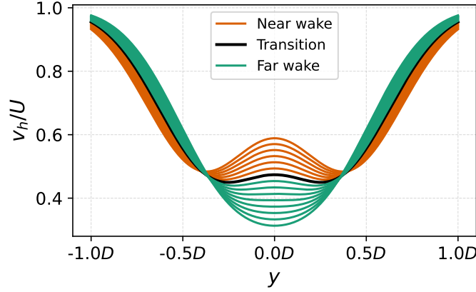
Figure 5. Double Gaussian curves (Eq. 6) in the near wake region (brown), at the transition point to far wake (black) and in the far wake (green) for A = -0.50.5 , \sigma = 0.3 , d = 0.1 and reducing b_1 = -b_2 , \mu_1 = -\mu_2 from 0.4 to 0.26 across y from -1 D to 1 D .
