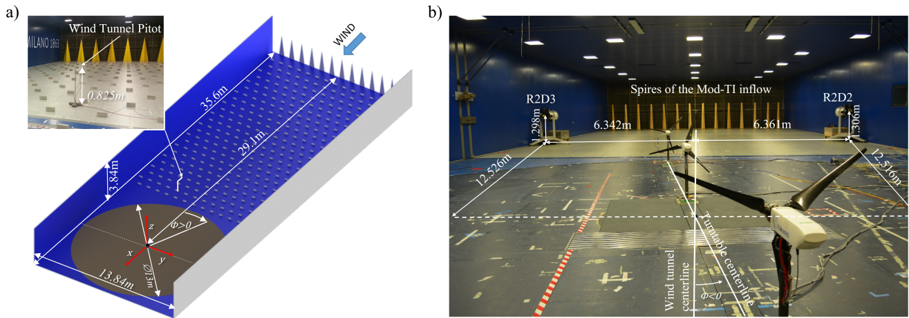
Figure 1. Main dimensions of the test section of the POLIMI wind tunnel, including the distance of the turntable center from the inlet (a) ; Boundary layer test section equipped with the spires used to simulate the Mod-TI inflow (b) . Wind turbine and flow-measurement device positions are measured relative to the depicted reference frame, whose origin lies at the turntable center (a) . Boundary layer test section equipped with the spires used to simulate the Mod-TI inflow; note that the turntable angle \Phi shown in this figure panel is negative (b). ]
