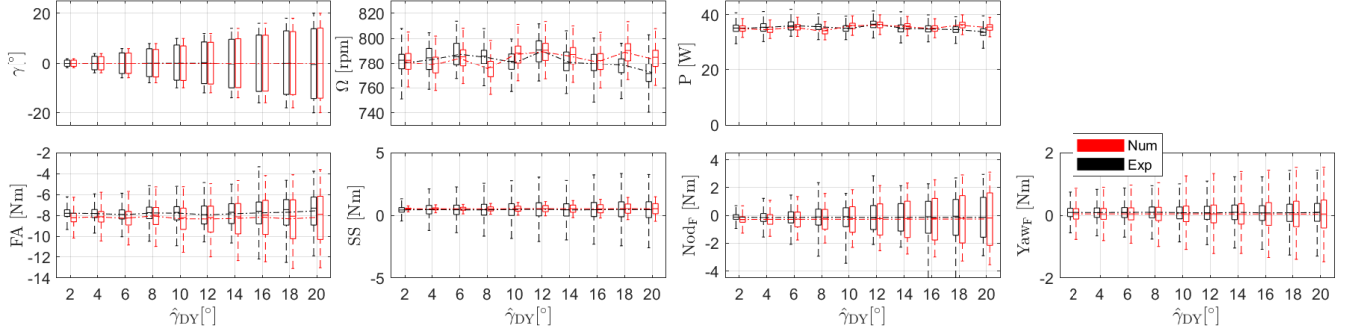
Figure A4. Dataset “Wind turbine data under steady wind direction”. Comparison between experimental (black) data and numerical (red) predictions for DY operation ( f_{DY} = 0.75 Hz) of WT1 under Mod-TI below-rated inflow conditions and varying amplitude \hat{\gamma}_{DY} (test IDs: [1069 1081 1094 1106 1120 1126 1131 1134 1139 1141]).
