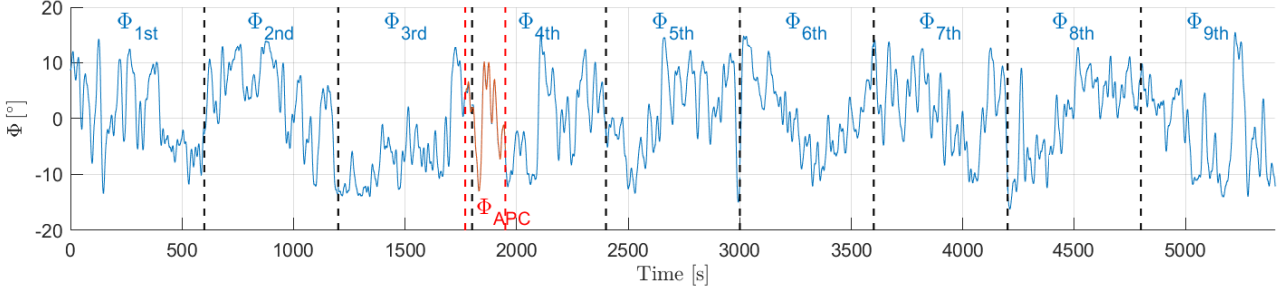
Figure 10. The 90-minute time history of the rotation imposed on the turntable during experiments with dynamically varying wind direction. The 10-minute blocks used for the power-boosting experiments are shown in blue and are separated by vertical black dashed lines. The 180 s block used for the APC experiments, labeled \Phi_{APC} , is shown in red.
