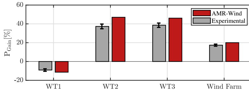
Figure A7. Dataset “Multiple wakes measurement with lidars”. Comparison of experimental measurements and AMR-Wind predictions of the power gain P_{\text{Gain}} relative to greedy control (ID 1), obtained by yaw-misaligning the two upstream turbines (ID 4) under Mod-TI below-rated inflow conditions. The error bars represent the uncertainty of the experimental measurements.
