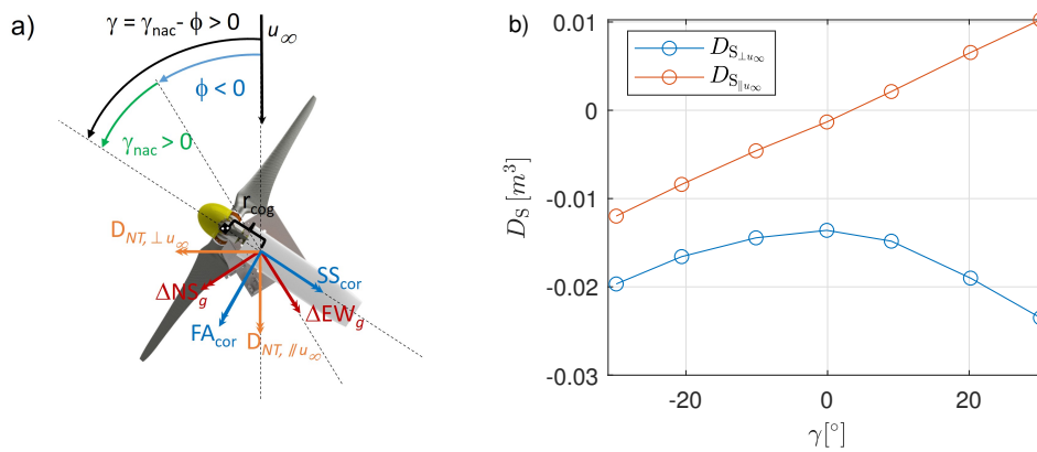
Figure 6. Schematic of the thrust calculation (a). Drag static moments of the G1 nacelle and tower as a function of the yaw misalignment (b).
